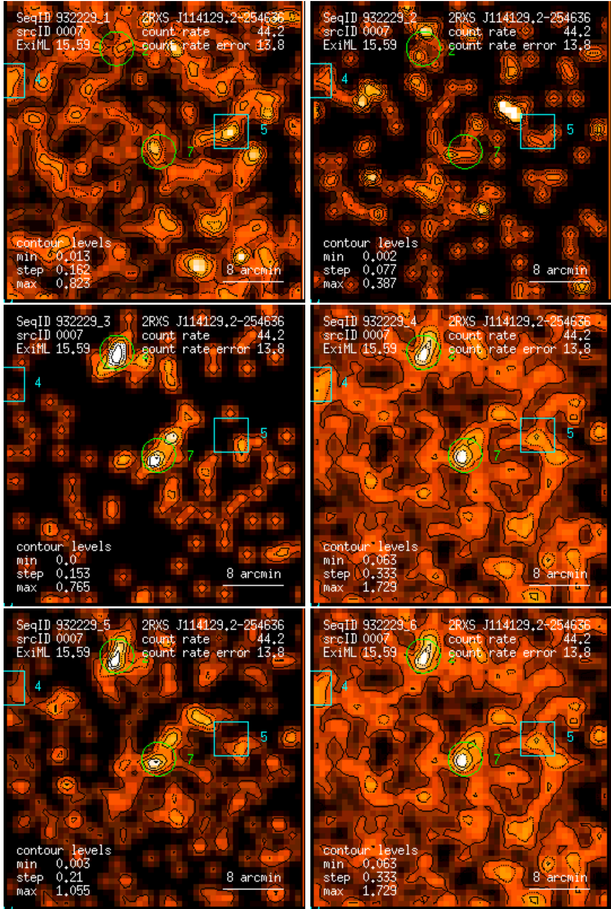
Figure 7: RASS 932229: detection 0007: band rate images, Gaussian filter: (1) PSPC channels 11 – 41, (2) 52 – 90, (3) 91 – 201, (4) 11 – 235, (5) 52 – 201, (6) 11 – 201. Broad band rates in counts/ks. Band rate contour levels in counts/ks/arcmin 2 .
