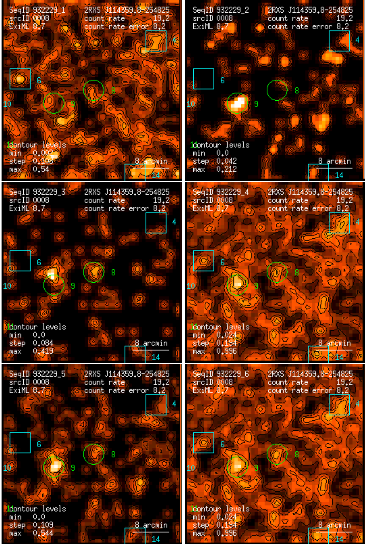
Figure 8: RASS 932229: detection 0008: band rate images, Gaussian filter: (1) PSPC channels 11 – 41, (2) 52 – 90, (3) 91 – 201, (4) 11 – 235, (5) 52 – 201, (6) 11 – 201. Broad band rates in counts/ks. Band rate contour levels in counts/ks/arcmin 2 .
