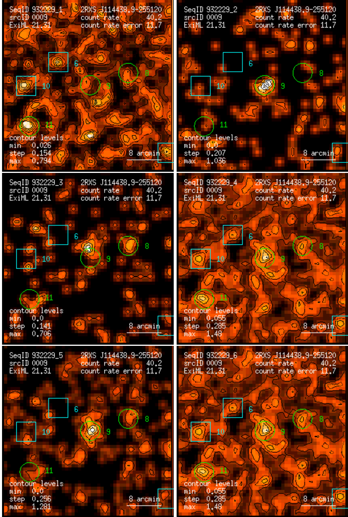
Figure 9: RASS 932229: detection 0009: band rate images, Gaussian filter: (1) PSPC channels 11 – 41, (2) 52 – 90, (3) 91 – 201, (4) 11 – 235, (5) 52 – 201, (6) 11 – 201. Broad band rates in counts/ks. Band rate contour levels in counts/ks/arcmin 2 .
