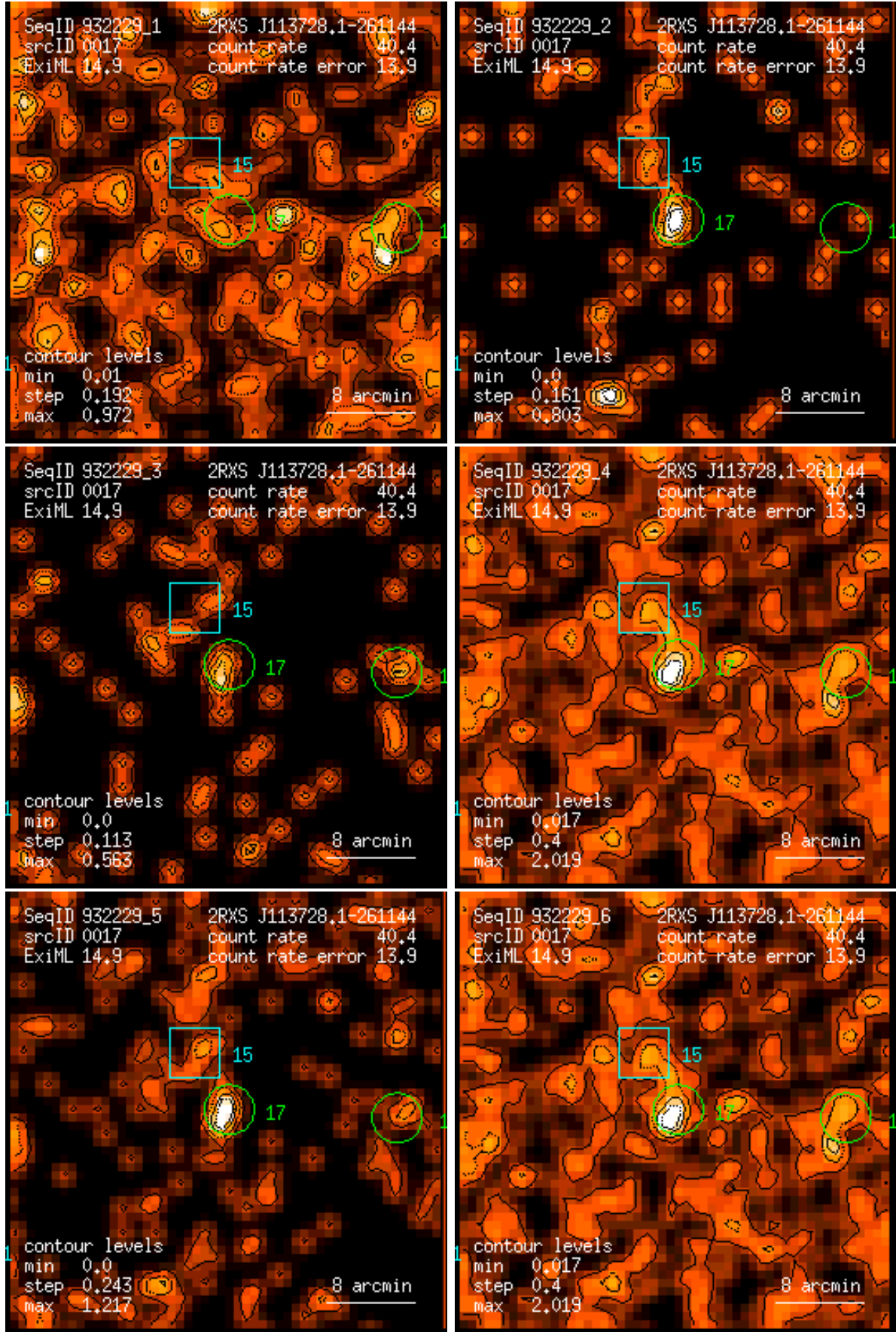
Figure 17: RASS 932229: detection 0017: band rate images, Gaussian filter: (1) PSPC channels 11 – 41, (2) 52 – 90, (3) 91 – 201, (4) 11 – 235, (5) 52 – 201, (6) 11 – 201. Broad band rates in counts/ks. Band rate contour levels in counts/ks/arcmin 2 .
