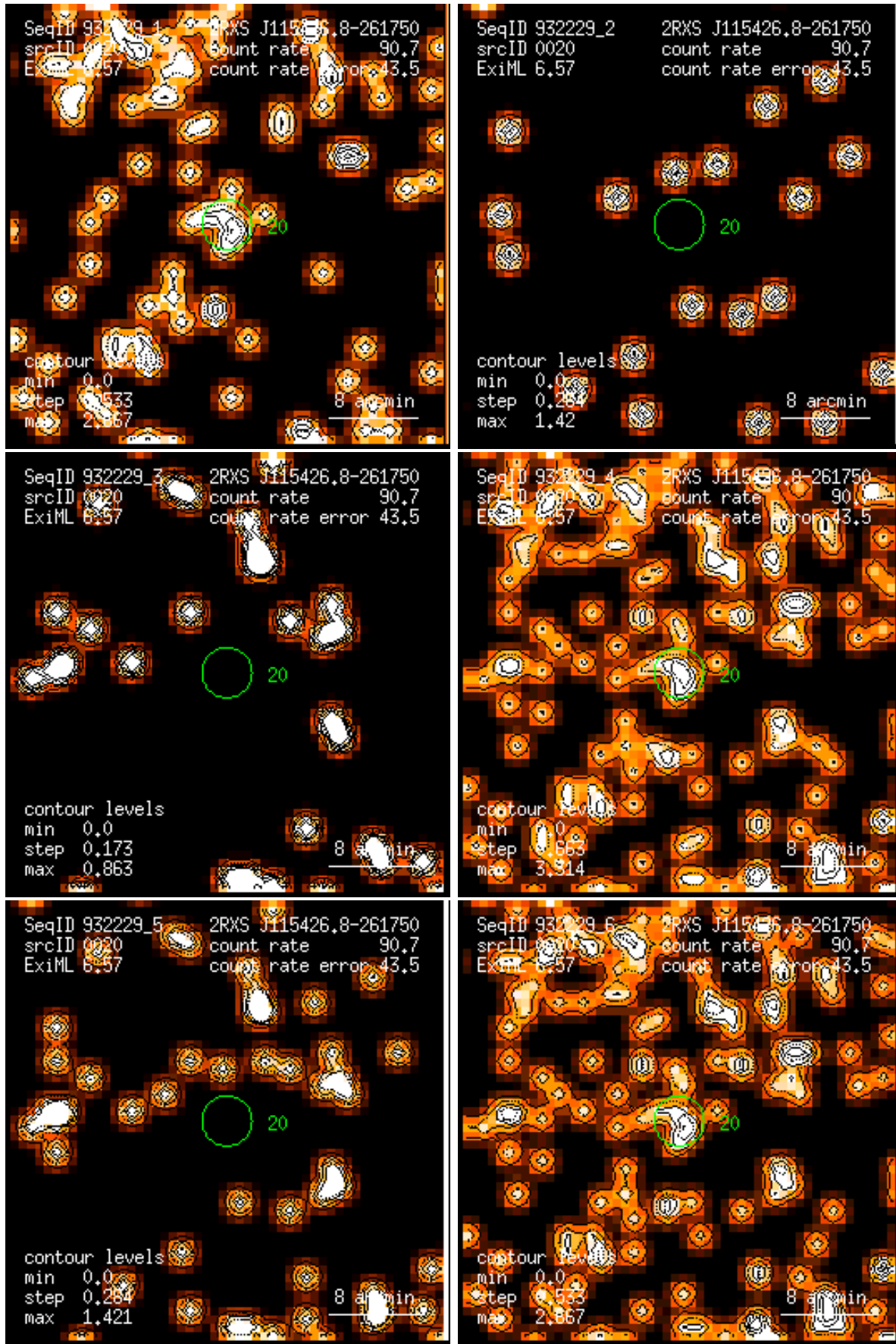
Figure 20: RASS 932229: detection 0020: band rate images, Gaussian filter: (1) PSPC channels 11 – 41, (2) 52 – 90, (3) 91 – 201, (4) 11 – 235, (5) 52 – 201, (6) 11 – 201. Broad band rates in counts/ks. Band rate contour levels in counts/ks/arcmin 2 .
