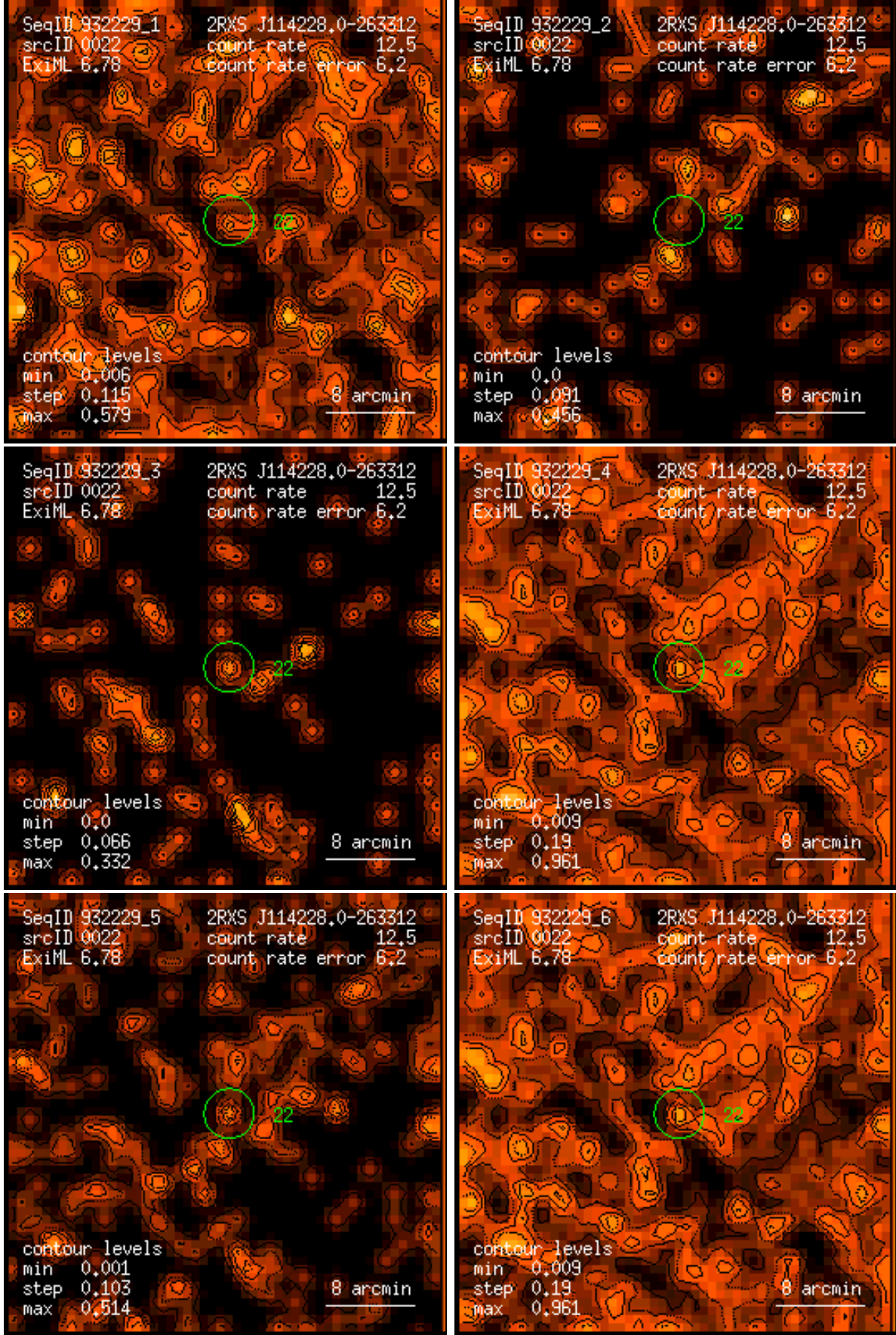
Figure 22: RASS 932229: detection 0022: band rate images, Gaussian filter: (1) PSPC channels 11 – 41, (2) 52 – 90, (3) 91 – 201, (4) 11 – 235, (5) 52 – 201, (6) 11 – 201. Broad band rates in counts/ks. Band rate contour levels in counts/ks/arcmin 2 .
