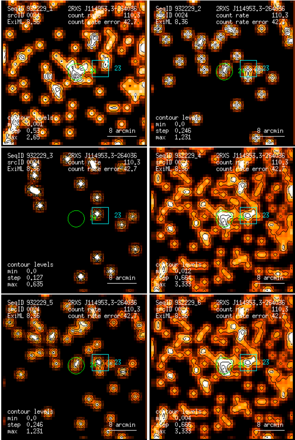
Figure 24: RASS 932229: detection 0024: band rate images, Gaussian filter: (1) PSPC channels 11 – 41, (2) 52 – 90, (3) 91 – 201, (4) 11 – 235, (5) 52 – 201, (6) 11 – 201. Broad band rates in counts/ks. Band rate contour levels in counts/ks/arcmin 2 .
