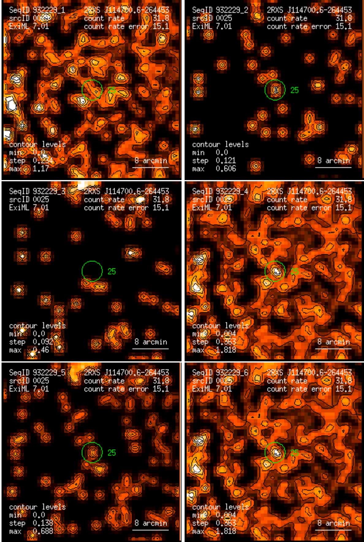
Figure 25: RASS 932229: detection 0025: band rate images, Gaussian filter: (1) PSPC channels 11 – 41, (2) 52 – 90, (3) 91 – 201, (4) 11 – 235, (5) 52 – 201, (6) 11 – 201. Broad band rates in counts/ks. Band rate contour levels in counts/ks/arcmin 2 .
