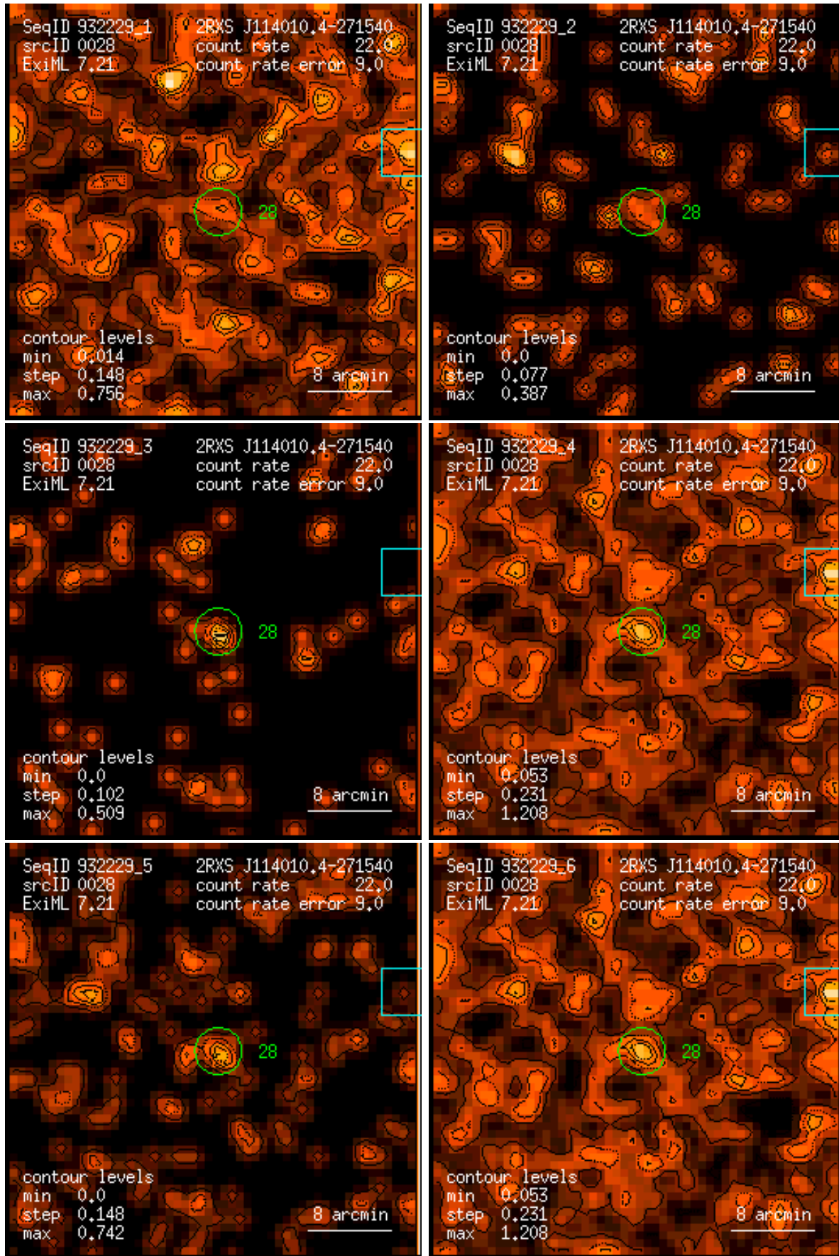
Figure 28: RASS 932229: detection 0028: band rate images, Gaussian filter: (1) PSPC channels 11 – 41, (2) 52 – 90, (3) 91 – 201, (4) 11 – 235, (5) 52 – 201, (6) 11 – 201. Broad band rates in counts/ks. Band rate contour levels in counts/ks/arcmin 2 .
