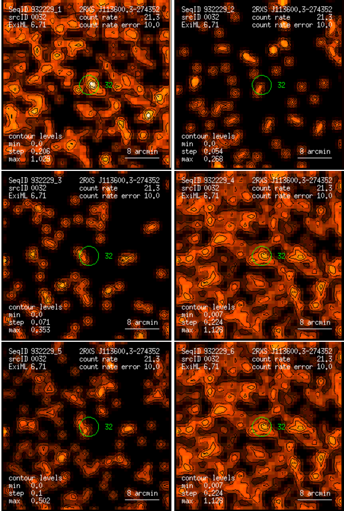
Figure 32: RASS 932229: detection 0032: band rate images, Gaussian filter: (1) PSPC channels 11 – 41, (2) 52 – 90, (3) 91 – 201, (4) 11 – 235, (5) 52 – 201, (6) 11 – 201. Broad band rates in counts/ks. Band rate contour levels in counts/ks/arcmin 2 .
