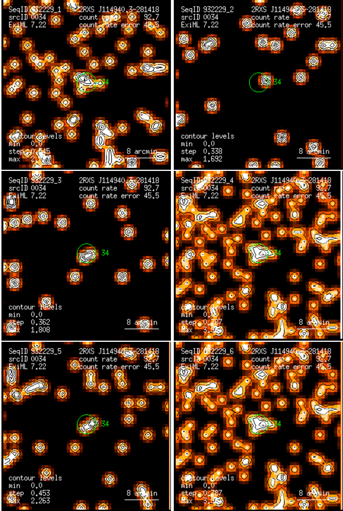
Figure 34: RASS 932229: detection 0034: band rate images, Gaussian filter: (1) PSPC channels 11 – 41, (2) 52 – 90, (3) 91 – 201, (4) 11 – 235, (5) 52 – 201, (6) 11 – 201. Broad band rates in counts/ks. Band rate contour levels in counts/ks/arcmin 2 .
