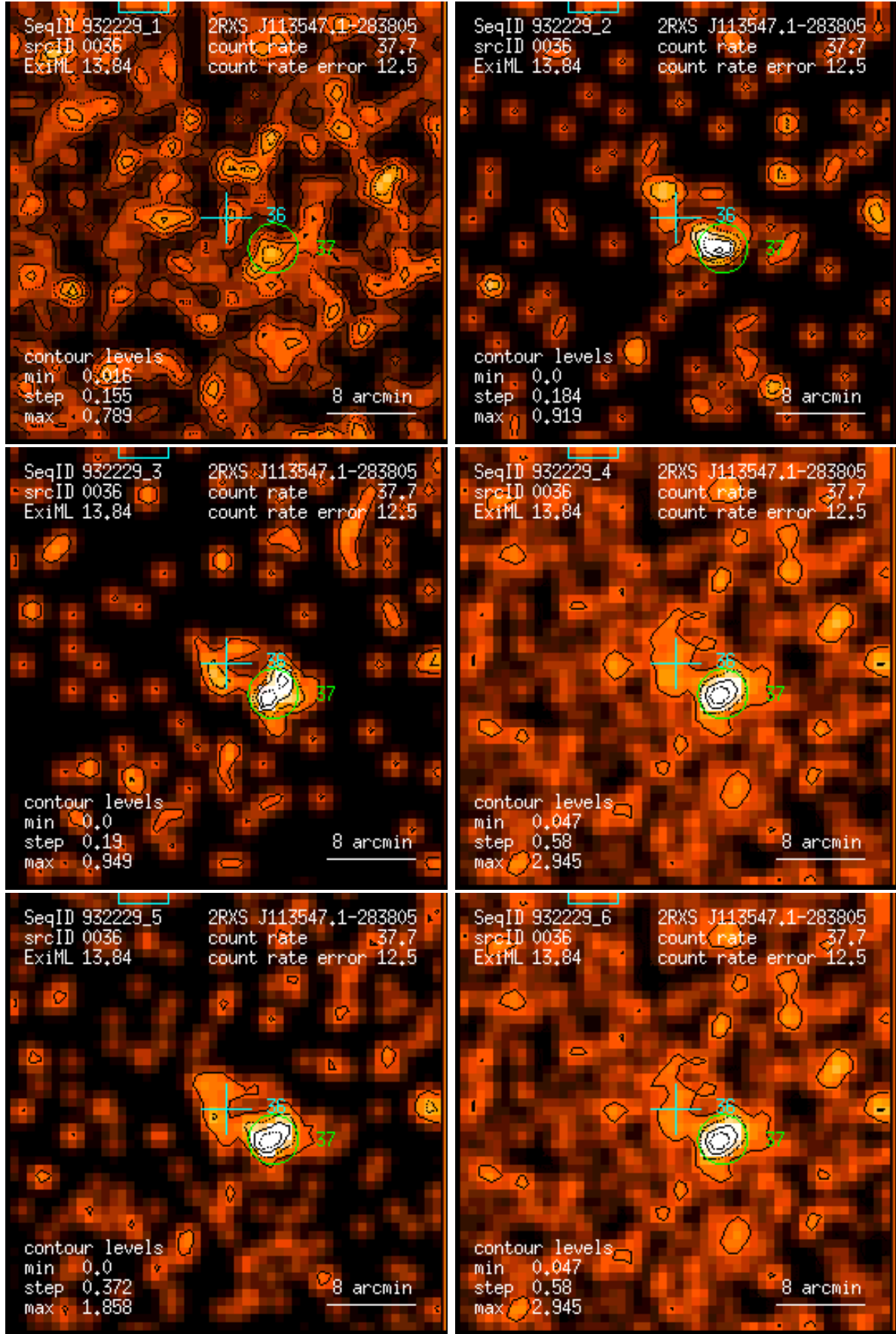
Figure 36: RASS 932229: detection 0036: band rate images, Gaussian filter: (1) PSPC channels 11 – 41, (2) 52 – 90, (3) 91 – 201, (4) 11 – 235, (5) 52 – 201, (6) 11 – 201. Broad band rates in counts/ks. Band rate contour levels in counts/ks/arcmin 2 .
