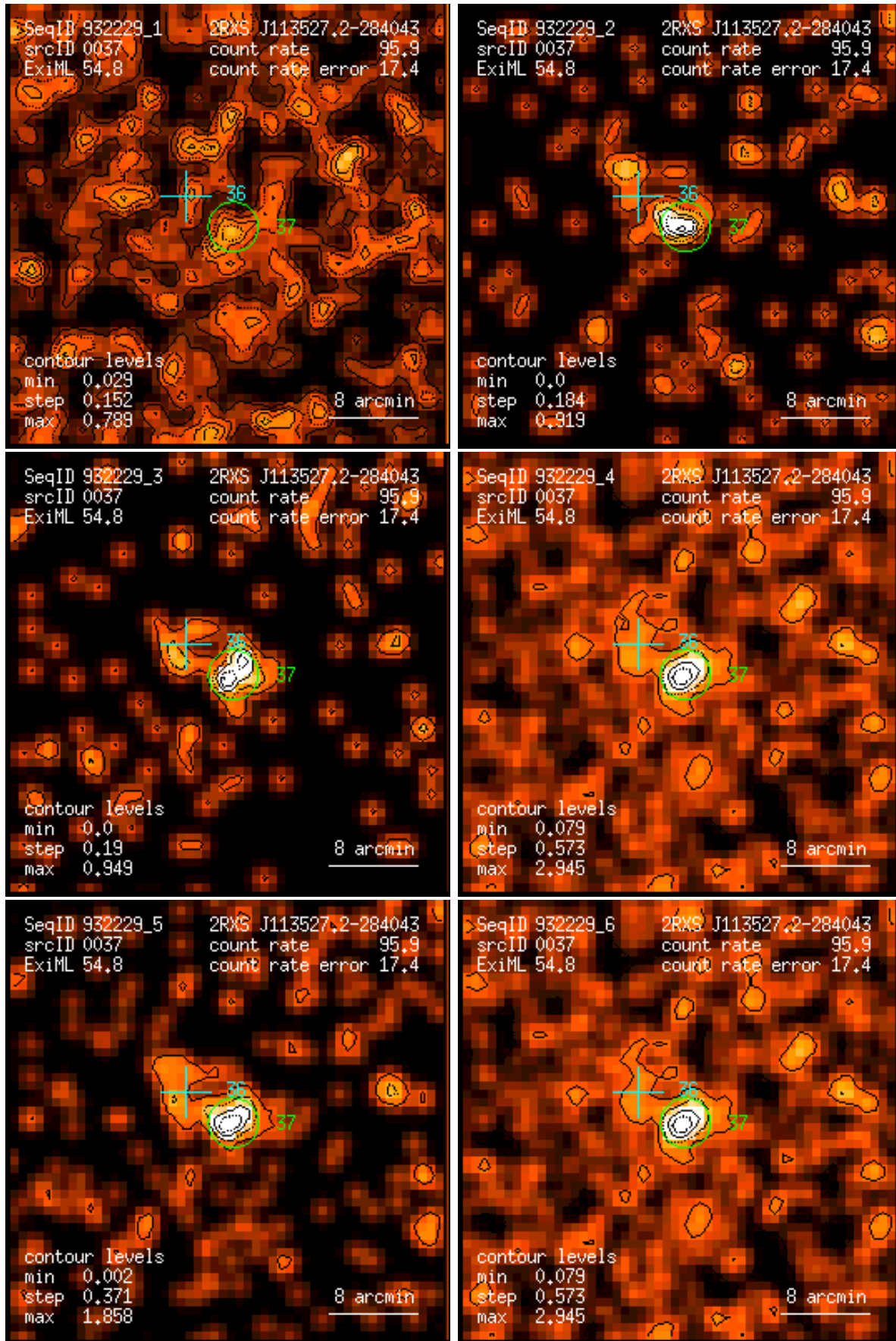
Figure 37: RASS 932229: detection 0037: band rate images, Gaussian filter: (1) PSPC channels 11 – 41, (2) 52 – 90, (3) 91 – 201, (4) 11 – 235, (5) 52 – 201, (6) 11 – 201. Broad band rates in counts/ks. Band rate contour levels in counts/ks/arcmin 2 .
