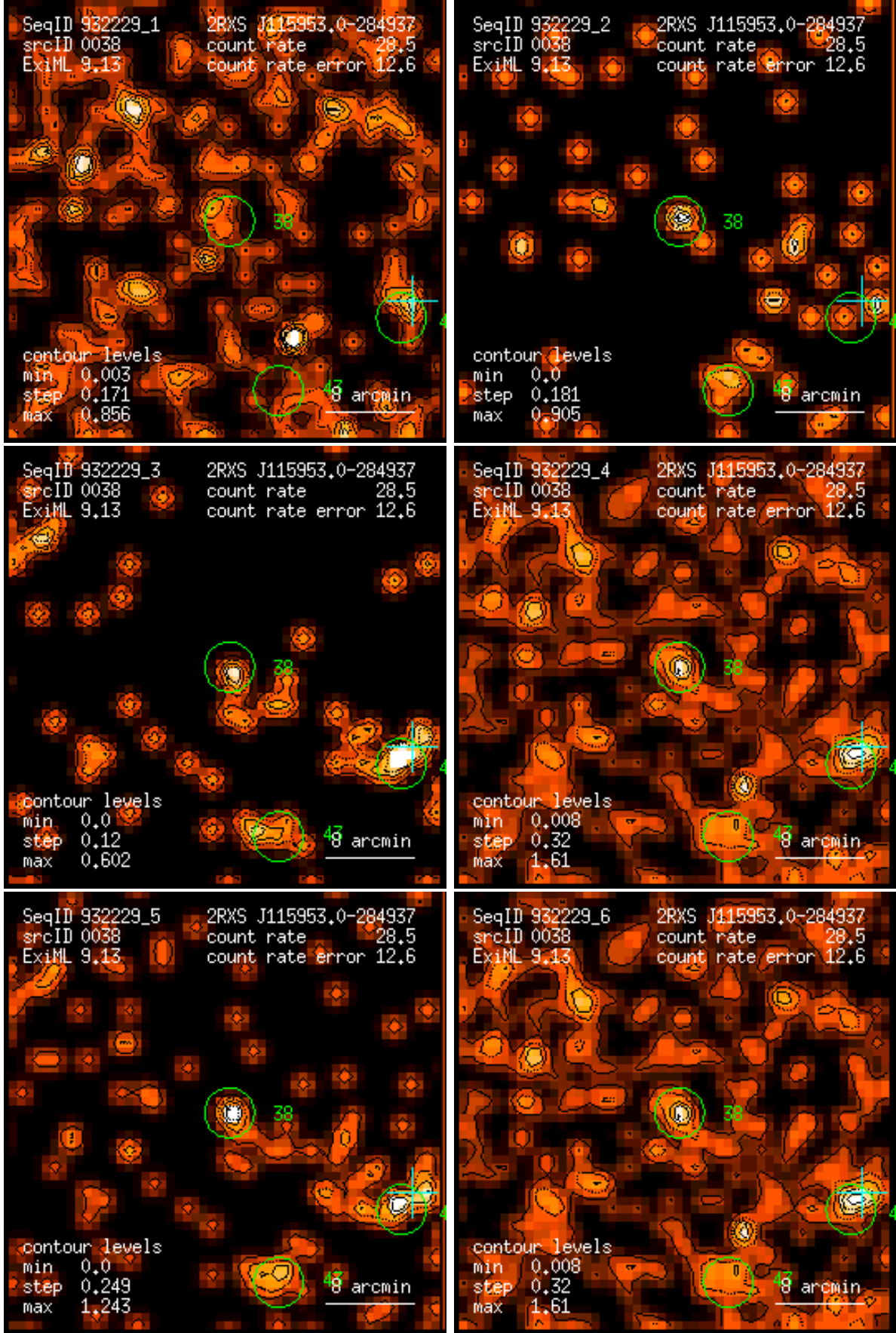
Figure 38: RASS 932229: detection 0038: band rate images, Gaussian filter: (1) PSPC channels 11 – 41, (2) 52 – 90, (3) 91 – 201, (4) 11 – 235, (5) 52 – 201, (6) 11 – 201. Broad band rates in counts/ks. Band rate contour levels in counts/ks/arcmin 2 .
