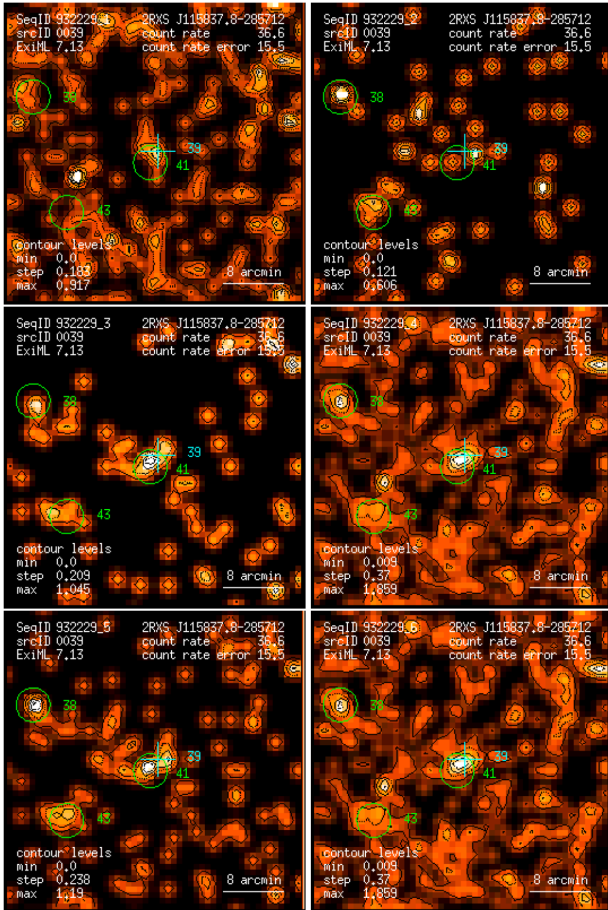
Figure 39: RASS 932229: detection 0039: band rate images, Gaussian filter: (1) PSPC channels 11 – 41, (2) 52 – 90, (3) 91 – 201, (4) 11 – 235, (5) 52 – 201, (6) 11 – 201. Broad band rates in counts/ks. Band rate contour levels in counts/ks/arcmin 2 .
