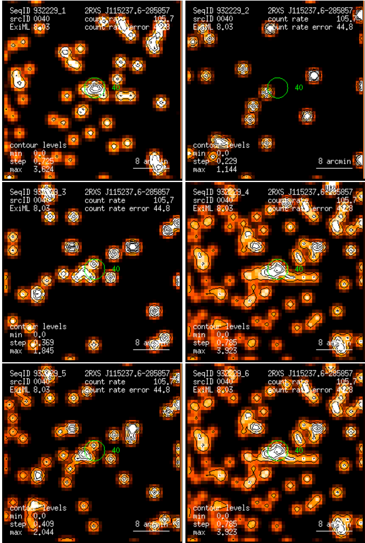
Figure 40: RASS 932229: detection 0040: band rate images, Gaussian filter: (1) PSPC channels 11 – 41, (2) 52 – 90, (3) 91 – 201, (4) 11 – 235, (5) 52 – 201, (6) 11 – 201. Broad band rates in counts/ks. Band rate contour levels in counts/ks/arcmin 2 .
