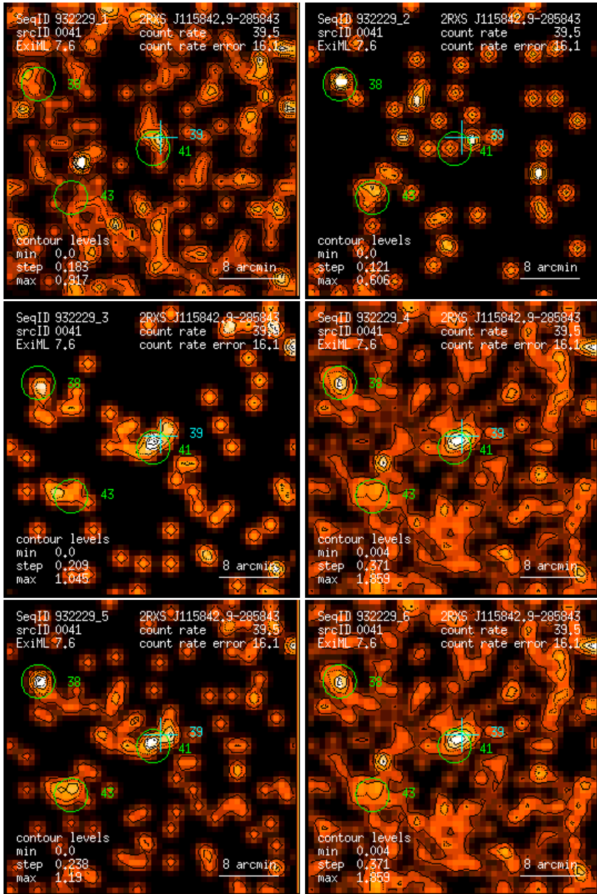
Figure 41: RASS 932229: detection 0041: band rate images, Gaussian filter: (1) PSPC channels 11 – 41, (2) 52 – 90, (3) 91 – 201, (4) 11 – 235, (5) 52 – 201, (6) 11 – 201. Broad band rates in counts/ks. Band rate contour levels in counts/ks/arcmin 2 .
