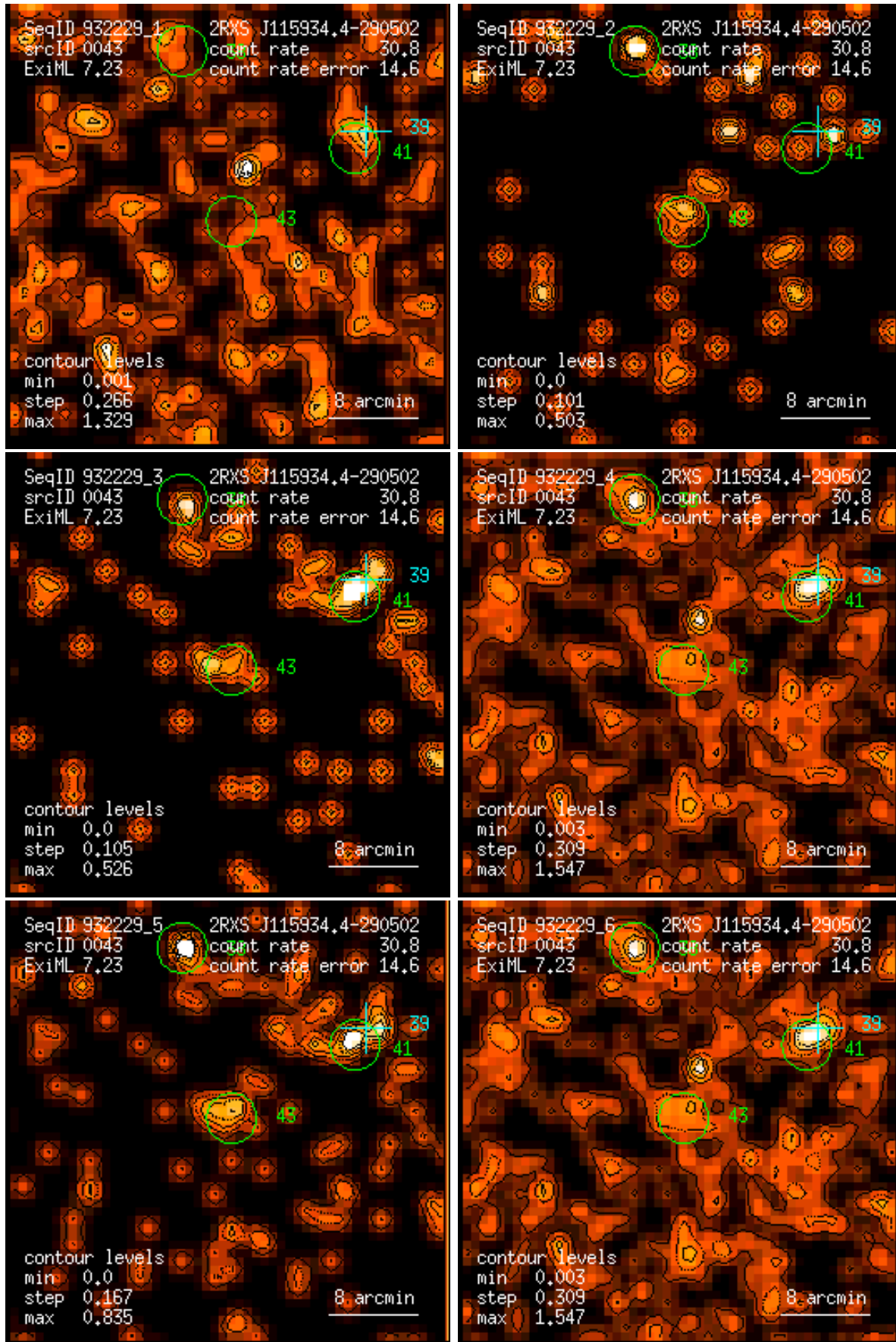
Figure 43: RASS 932229: detection 0043: band rate images, Gaussian filter: (1) PSPC channels 11 – 41, (2) 52 – 90, (3) 91 – 201, (4) 11 – 235, (5) 52 – 201, (6) 11 – 201. Broad band rates in counts/ks. Band rate contour levels in counts/ks/arcmin 2 .
