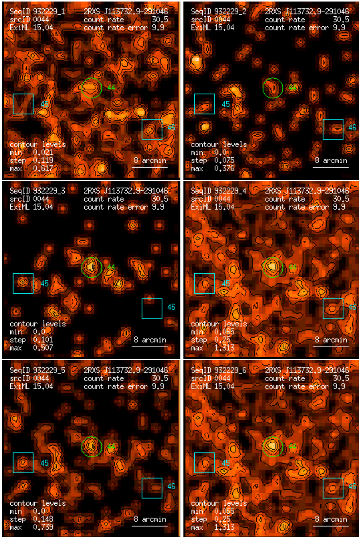
Figure 44: RASS 932229: detection 0044: band rate images, Gaussian filter: (1) PSPC channels 11 – 41, (2) 52 – 90, (3) 91 – 201, (4) 11 – 235, (5) 52 – 201, (6) 11 – 201. Broad band rates in counts/ks. Band rate contour levels in counts/ks/arcmin 2 .
