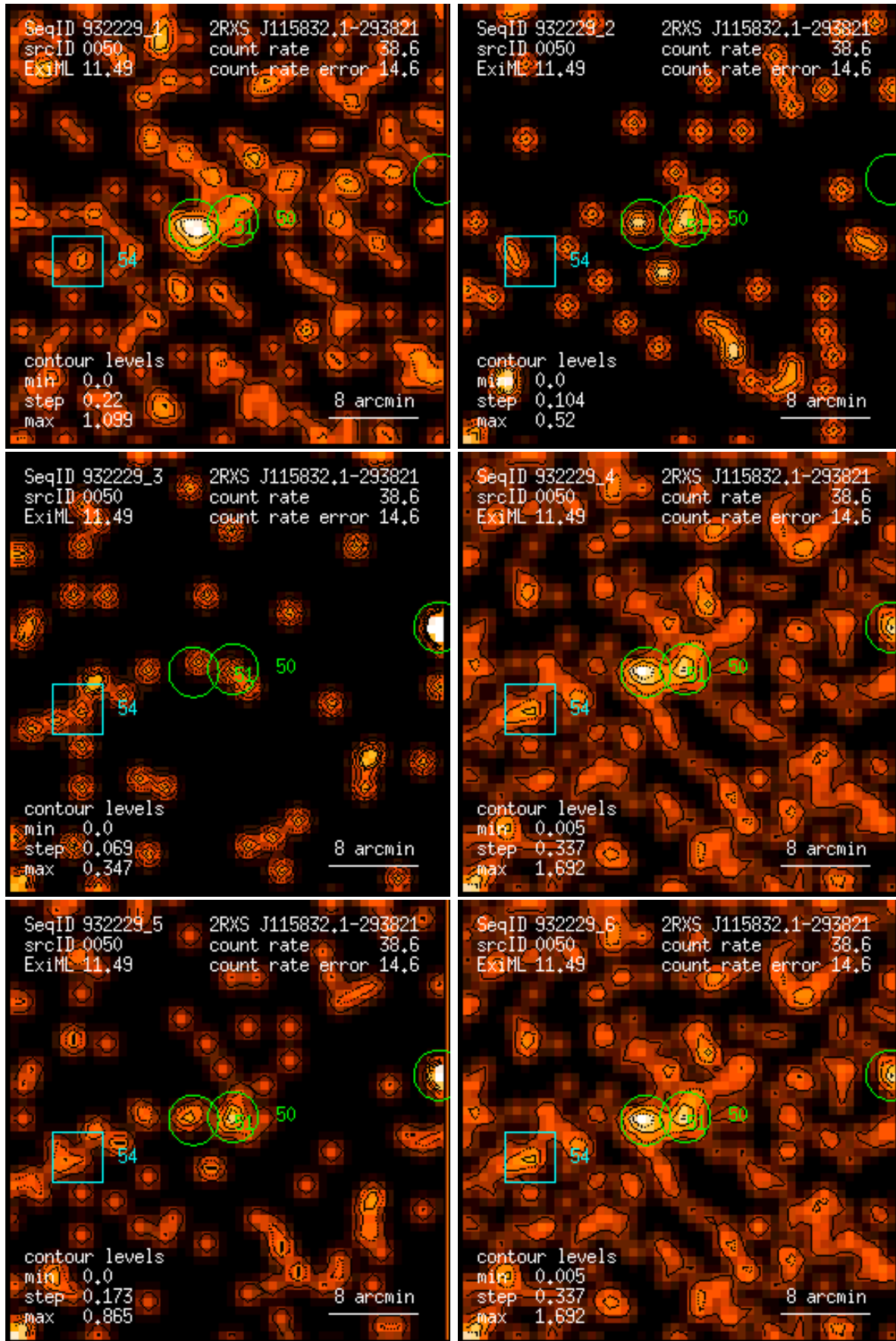
Figure 50: RASS 932229: detection 0050: band rate images, Gaussian filter: (1) PSPC channels 11 – 41, (2) 52 – 90, (3) 91 – 201, (4) 11 – 235, (5) 52 – 201, (6) 11 – 201. Broad band rates in counts/ks. Band rate contour levels in counts/ks/arcmin 2 .
