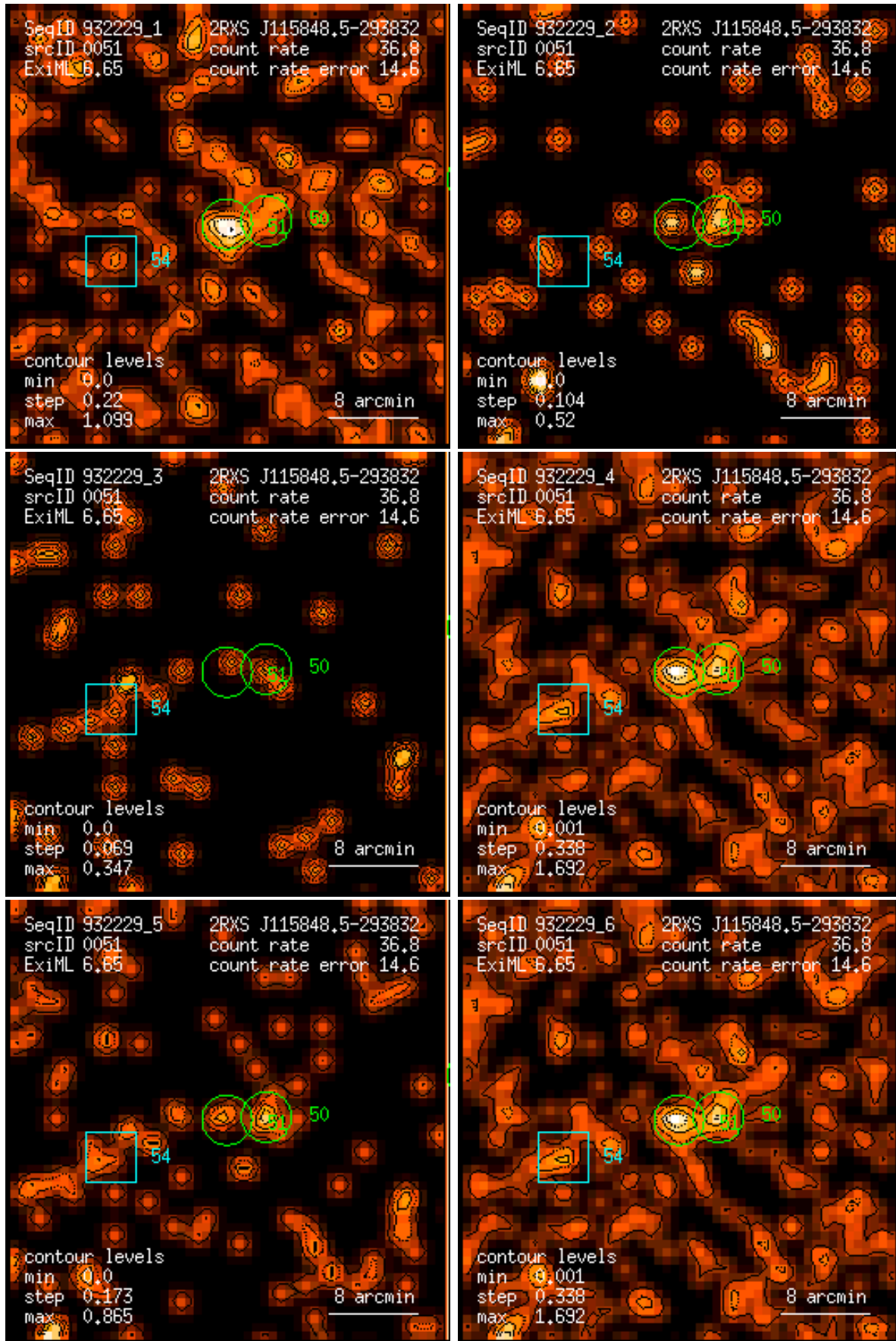
Figure 51: RASS 932229: detection 0051: band rate images, Gaussian filter: (1) PSPC channels 11 – 41, (2) 52 – 90, (3) 91 – 201, (4) 11 – 235, (5) 52 – 201, (6) 11 – 201. Broad band rates in counts/ks. Band rate contour levels in counts/ks/arcmin 2 .
