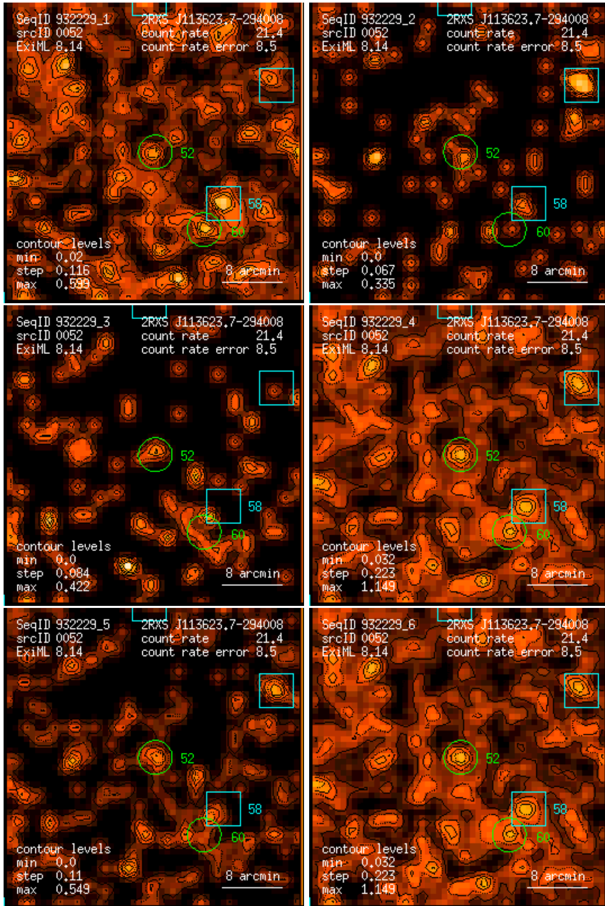
Figure 52: RASS 932229: detection 0052: band rate images, Gaussian filter: (1) PSPC channels 11 – 41, (2) 52 – 90, (3) 91 – 201, (4) 11 – 235, (5) 52 – 201, (6) 11 – 201. Broad band rates in counts/ks. Band rate contour levels in counts/ks/arcmin 2 .
