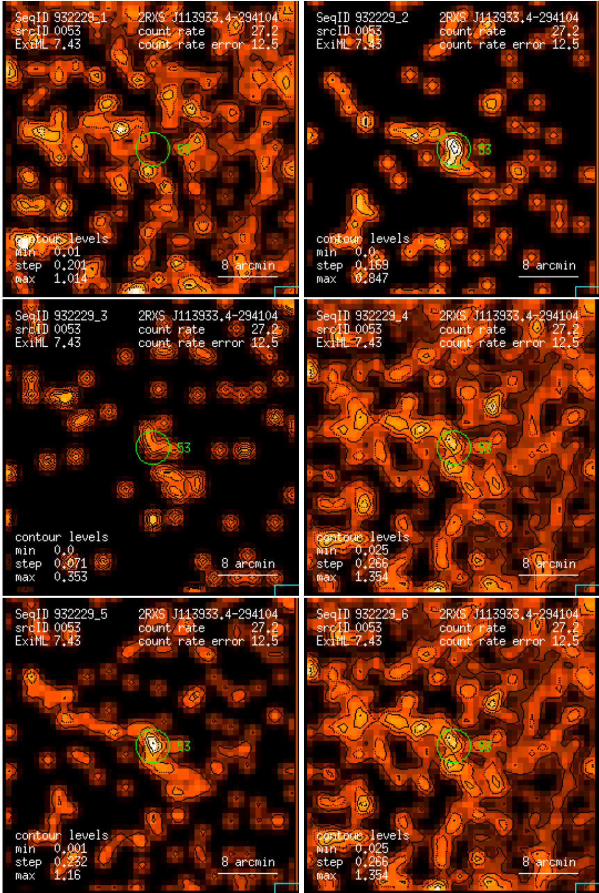
Figure 53: RASS 932229: detection 0053: band rate images, Gaussian filter: (1) PSPC channels 11 – 41, (2) 52 – 90, (3) 91 – 201, (4) 11 – 235, (5) 52 – 201, (6) 11 – 201. Broad band rates in counts/ks. Band rate contour levels in counts/ks/arcmin 2 .
