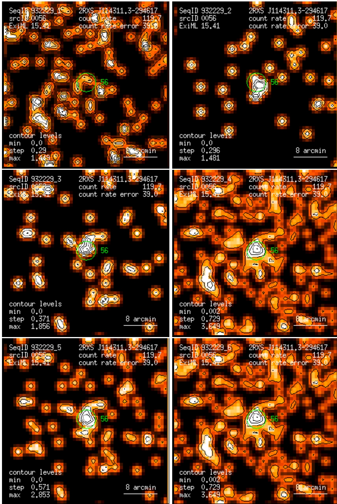
Figure 56: RASS 932229: detection 0056: band rate images, Gaussian filter: (1) PSPC channels 11 – 41, (2) 52 – 90, (3) 91 – 201, (4) 11 – 235, (5) 52 – 201, (6) 11 – 201. Broad band rates in counts/ks. Band rate contour levels in counts/ks/arcmin 2 .
