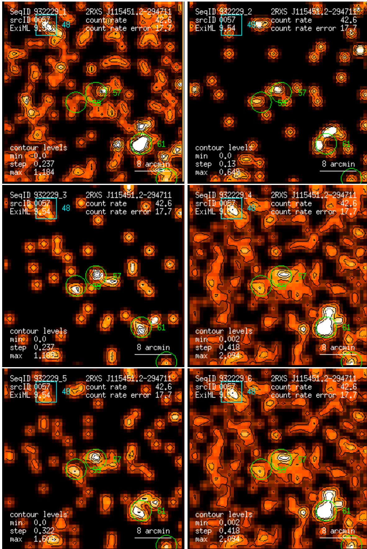
Figure 57: RASS 932229: detection 0057: band rate images, Gaussian filter: (1) PSPC channels 11 – 41, (2) 52 – 90, (3) 91 – 201, (4) 11 – 235, (5) 52 – 201, (6) 11 – 201. Broad band rates in counts/ks. Band rate contour levels in counts/ks/arcmin 2 .
