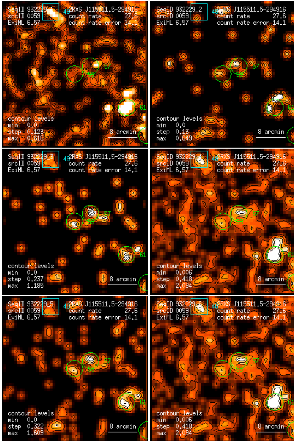
Figure 59: RASS 932229: detection 0059: band rate images, Gaussian filter: (1) PSPC channels 11 – 41, (2) 52 – 90, (3) 91 – 201, (4) 11 – 235, (5) 52 – 201, (6) 11 – 201. Broad band rates in counts/ks. Band rate contour levels in counts/ks/arcmin 2 .
