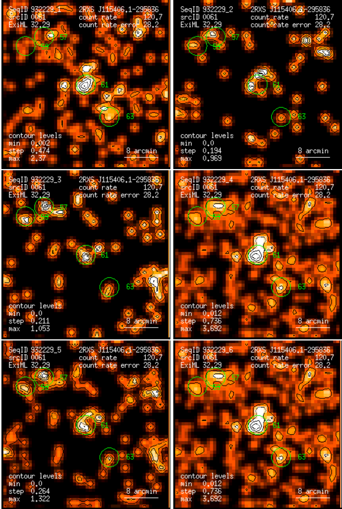
Figure 61: RASS 932229: detection 0061: band rate images, Gaussian filter: (1) PSPC channels 11 – 41, (2) 52 – 90, (3) 91 – 201, (4) 11 – 235, (5) 52 – 201, (6) 11 – 201. Broad band rates in counts/ks. Band rate contour levels in counts/ks/arcmin 2 .
