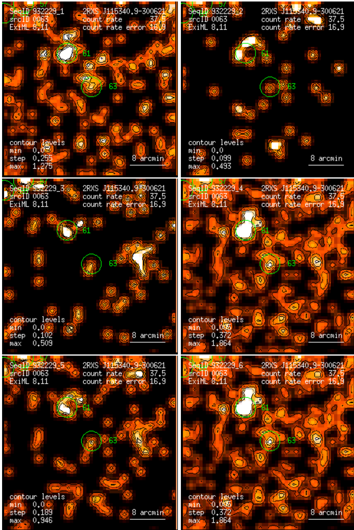
Figure 63: RASS 932229: detection 0063: band rate images, Gaussian filter: (1) PSPC channels 11 – 41, (2) 52 – 90, (3) 91 – 201, (4) 11 – 235, (5) 52 – 201, (6) 11 – 201. Broad band rates in counts/ks. Band rate contour levels in counts/ks/arcmin 2 .
