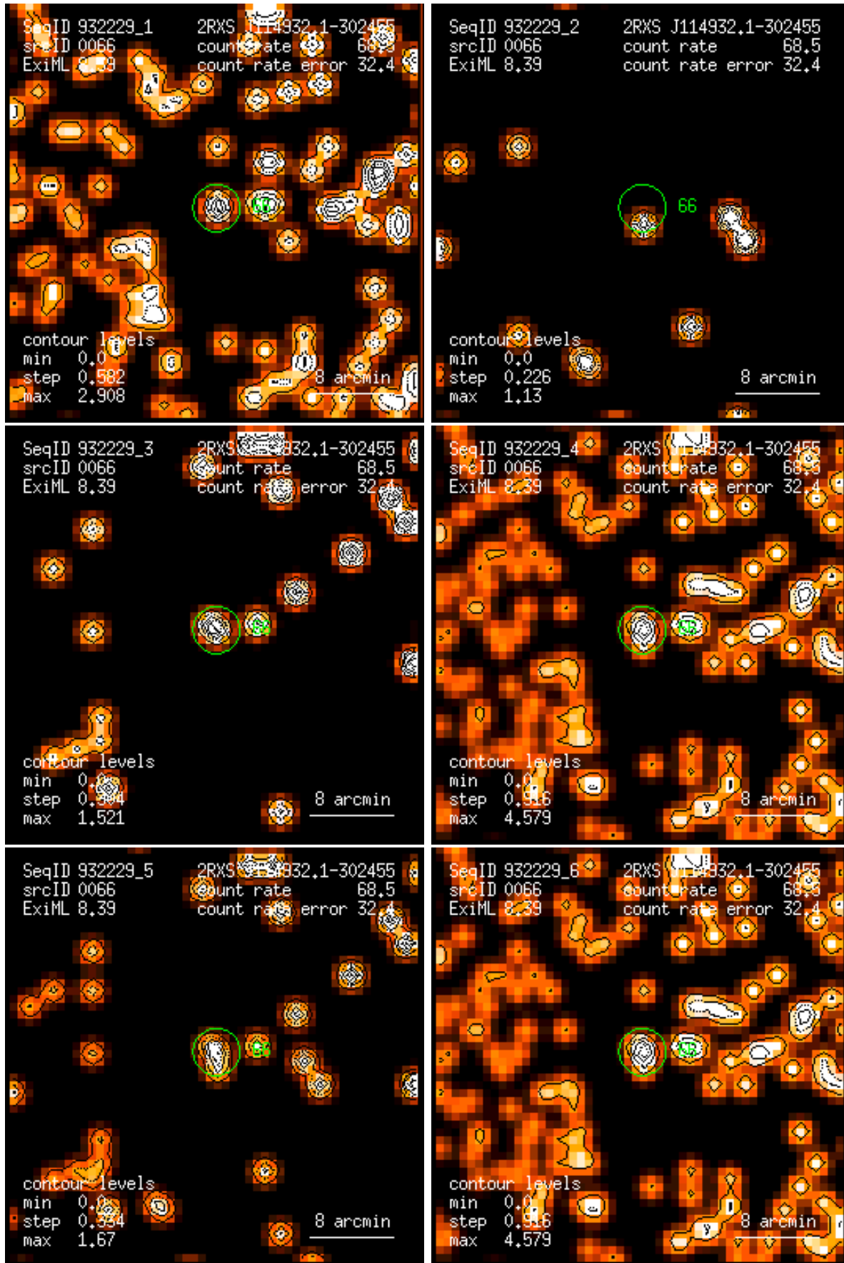
Figure 66: RASS 932229: detection 0066: band rate images, Gaussian filter: (1) PSPC channels 11 – 41, (2) 52 – 90, (3) 91 – 201, (4) 11 – 235, (5) 52 – 201, (6) 11 – 201. Broad band rates in counts/ks. Band rate contour levels in counts/ks/arcmin 2 .
