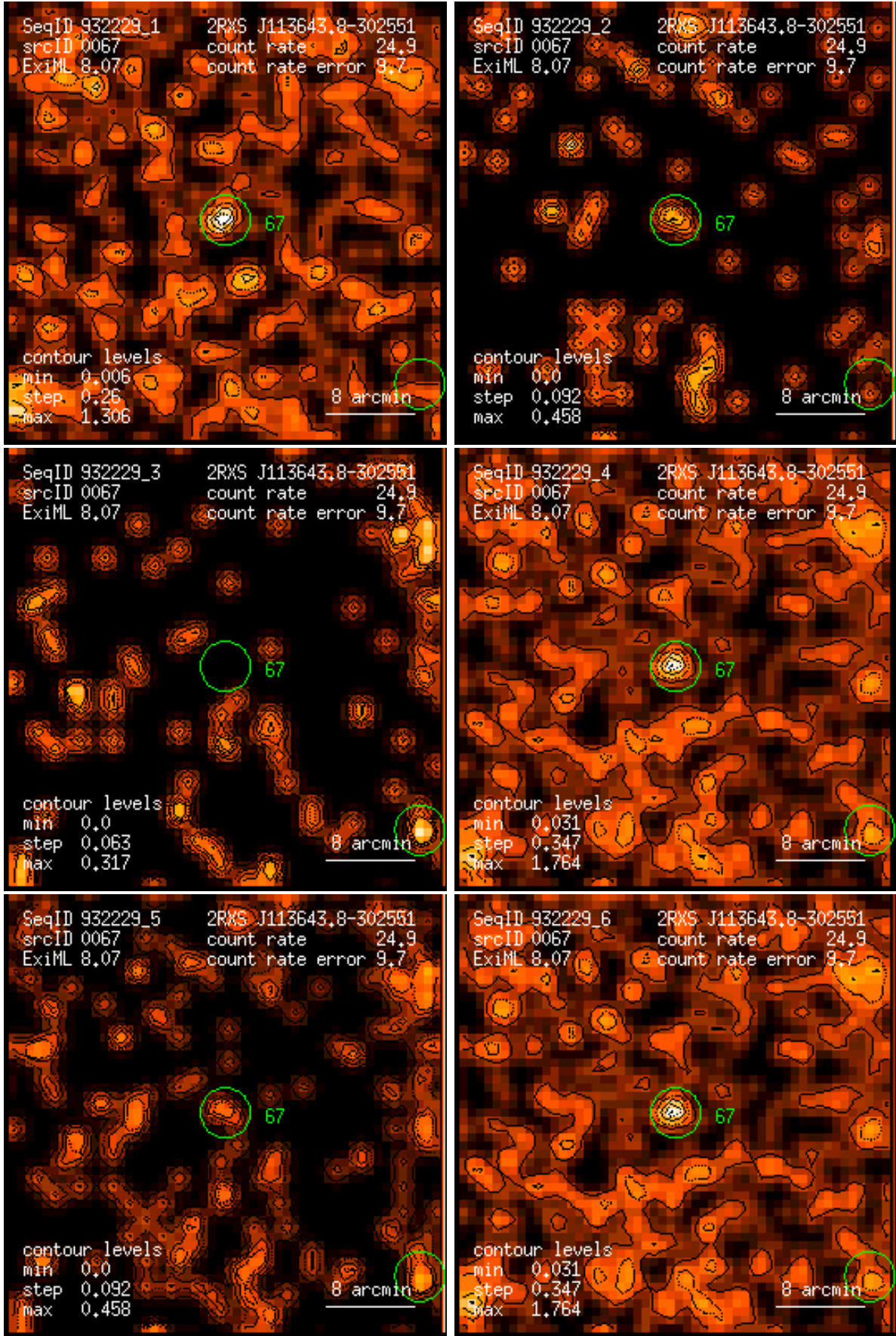
Figure 67: RASS 932229: detection 0067: band rate images, Gaussian filter: (1) PSPC channels 11 – 41, (2) 52 – 90, (3) 91 – 201, (4) 11 – 235, (5) 52 – 201, (6) 11 – 201. Broad band rates in counts/ks. Band rate contour levels in counts/ks/arcmin 2 .
