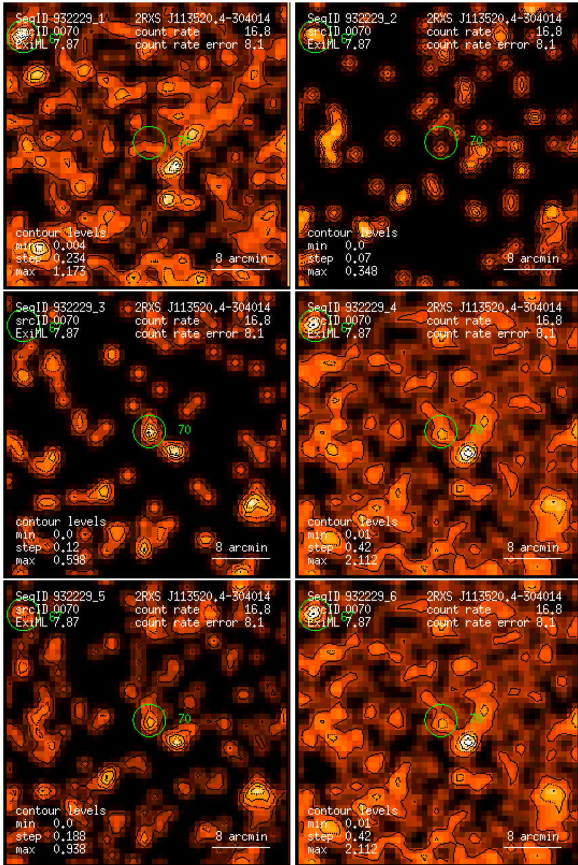
Figure 70: RASS 932229: detection 0070: band rate images, Gaussian filter: (1) PSPC channels 11 – 41, (2) 52 – 90, (3) 91 – 201, (4) 11 – 235, (5) 52 – 201, (6) 11 – 201. Broad band rates in counts/ks. Band rate contour levels in counts/ks/arcmin 2 .
