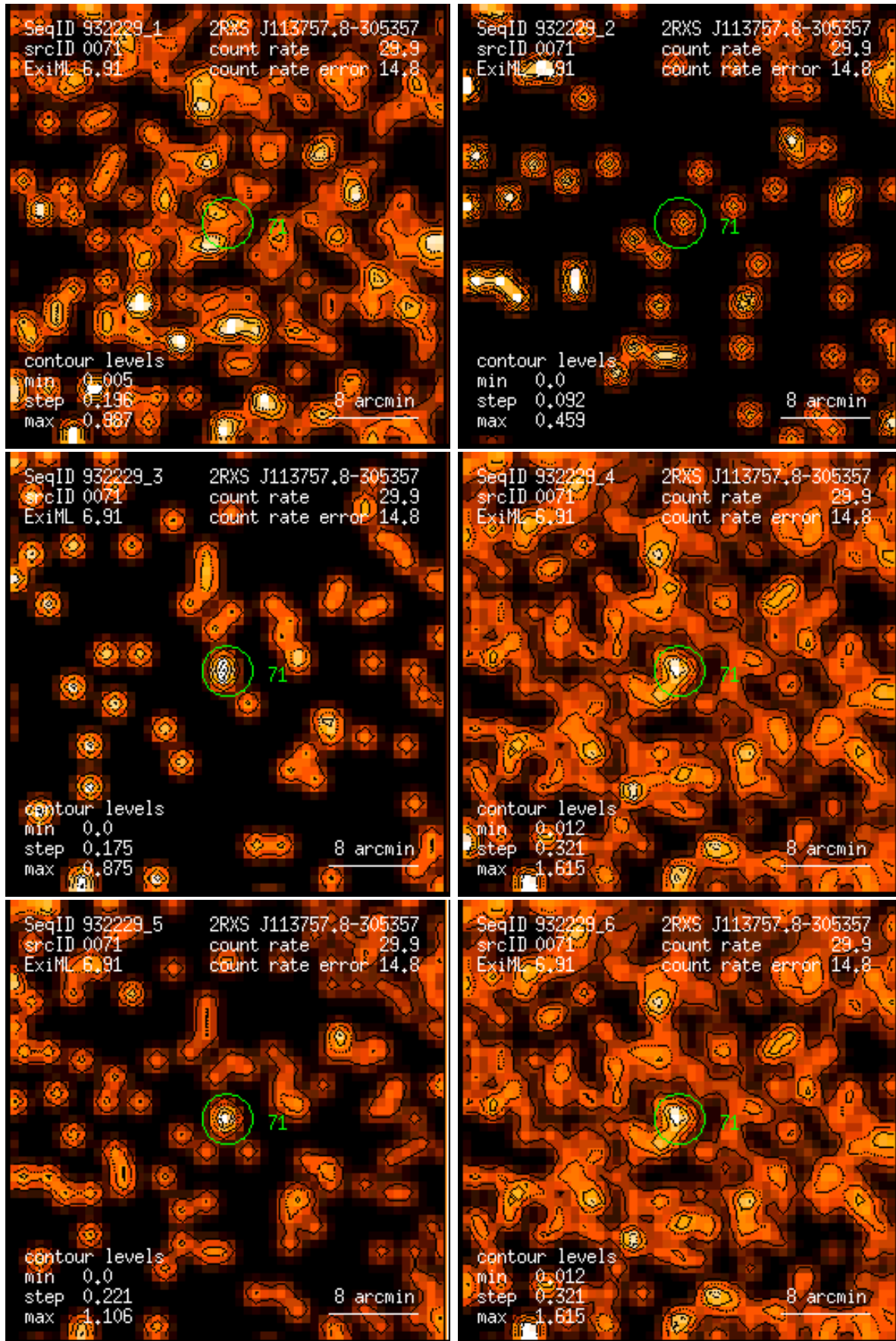
Figure 71: RASS 932229: detection 0071: band rate images, Gaussian filter: (1) PSPC channels 11 – 41, (2) 52 – 90, (3) 91 – 201, (4) 11 – 235, (5) 52 – 201, (6) 11 – 201. Broad band rates in counts/ks. Band rate contour levels in counts/ks/arcmin 2 .
