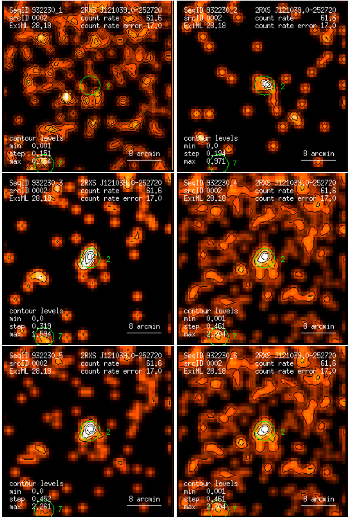
Figure 2: RASS 932230: detection 0002: band rate images, Gaussian filter: (1) PSPC channels 11 – 41, (2) 52 – 90, (3) 91 – 201, (4) 11 – 235, (5) 52 – 201, (6) 11 – 201. Broad band rates in counts/ks. Band rate contour levels in counts/ks/arcmin 2 .
