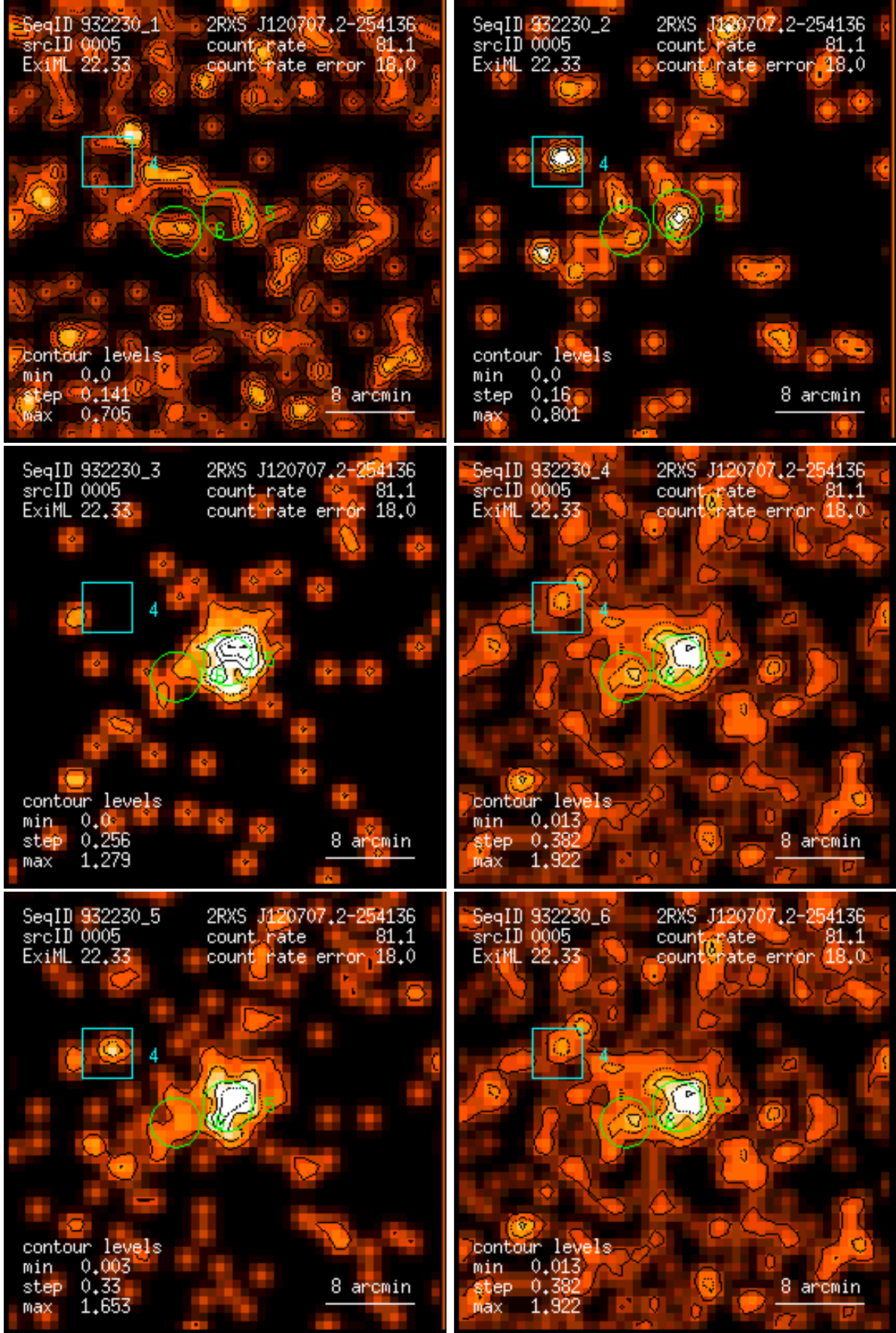
Figure 5: RASS 932230: detection 0005: band rate images, Gaussian filter: (1) PSPC channels 11 – 41, (2) 52 – 90, (3) 91 – 201, (4) 11 – 235, (5) 52 – 201, (6) 11 – 201. Broad band rates in counts/ks. Band rate contour levels in counts/ks/arcmin 2 .
