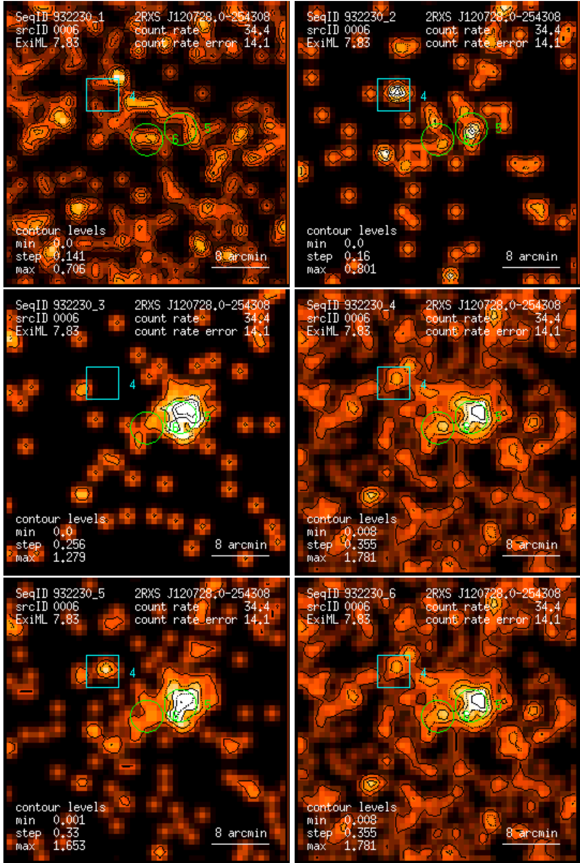
Figure 6: RASS 932230: detection 0006: band rate images, Gaussian filter: (1) PSPC channels 11 – 41, (2) 52 – 90, (3) 91 – 201, (4) 11 – 235, (5) 52 – 201, (6) 11 – 201. Broad band rates in counts/ks. Band rate contour levels in counts/ks/arcmin 2 .
