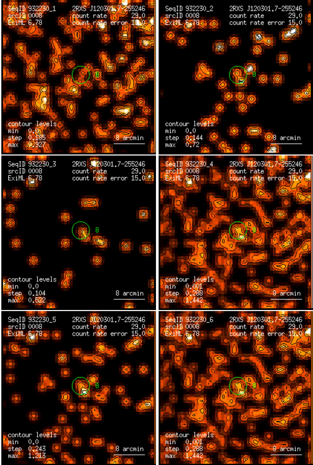
Figure 8: RASS 932230: detection 0008: band rate images, Gaussian filter: (1) PSPC channels 11 – 41, (2) 52 – 90, (3) 91 – 201, (4) 11 – 235, (5) 52 – 201, (6) 11 – 201. Broad band rates in counts/ks. Band rate contour levels in counts/ks/arcmin 2 .
