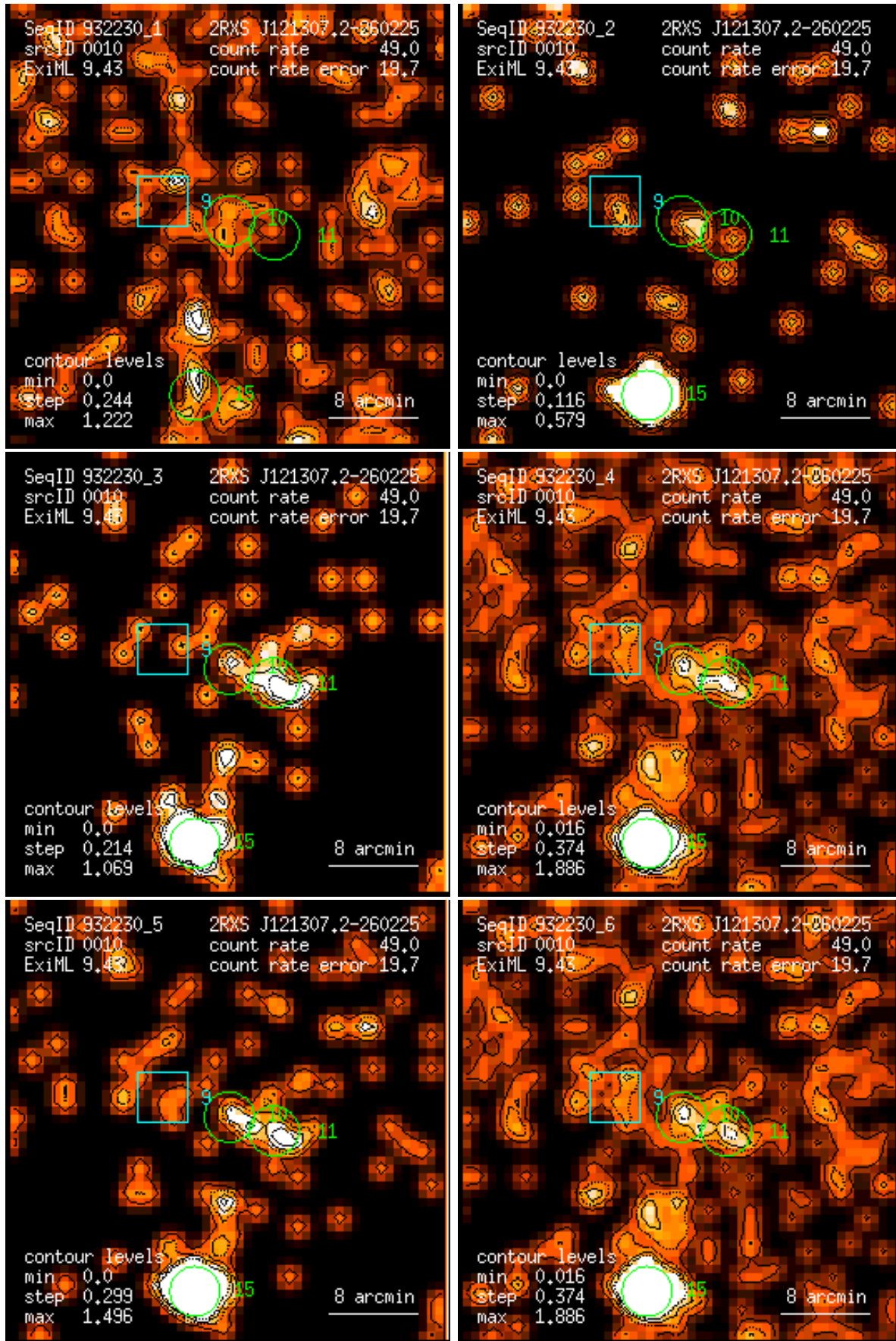
Figure 10: RASS 932230: detection 0010: band rate images, Gaussian filter: (1) PSPC channels 11 – 41, (2) 52 – 90, (3) 91 – 201, (4) 11 – 235, (5) 52 – 201, (6) 11 – 201. Broad band rates in counts/ks. Band rate contour levels in counts/ks/arcmin 2 .
