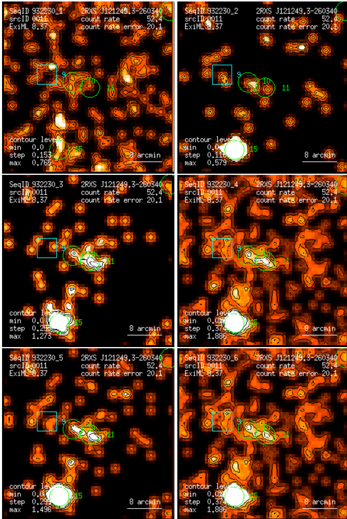
Figure 11: RASS 932230: detection 0011: band rate images, Gaussian filter: (1) PSPC channels 11 – 41, (2) 52 – 90, (3) 91 – 201, (4) 11 – 235, (5) 52 – 201, (6) 11 – 201. Broad band rates in counts/ks. Band rate contour levels in counts/ks/arcmin 2 .
