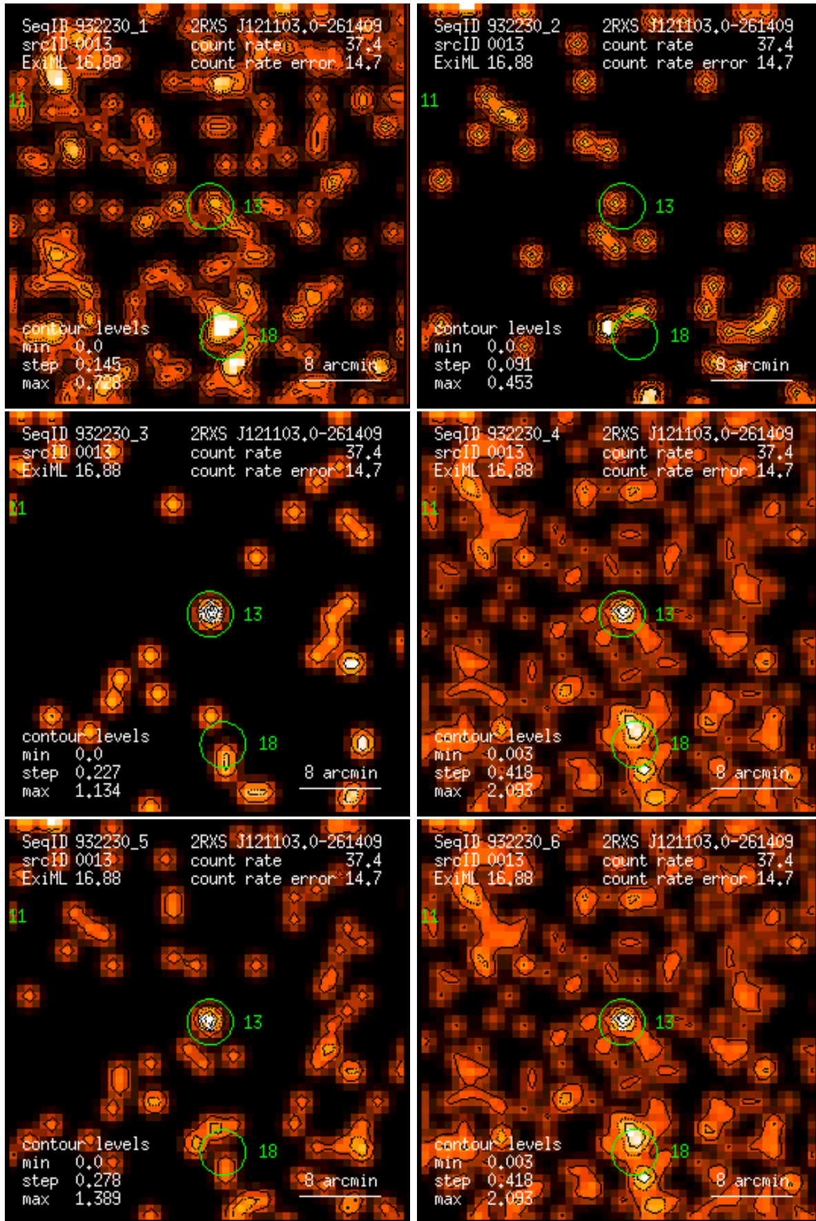
Figure 13: RASS 932230: detection 0013: band rate images, Gaussian filter: (1) PSPC channels 11 – 41, (2) 52 – 90, (3) 91 – 201, (4) 11 – 235, (5) 52 – 201, (6) 11 – 201. Broad band rates in counts/ks. Band rate contour levels in counts/ks/arcmin 2 .
