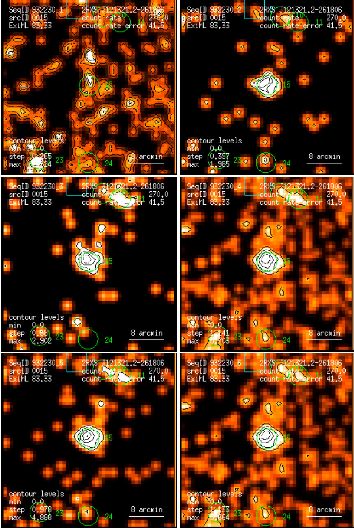
Figure 15: RASS 932230: detection 0015: band rate images, Gaussian filter: (1) PSPC channels 11 – 41, (2) 52 – 90, (3) 91 – 201, (4) 11 – 235, (5) 52 – 201, (6) 11 – 201. Broad band rates in counts/ks. Band rate contour levels in counts/ks/arcmin 2 .
