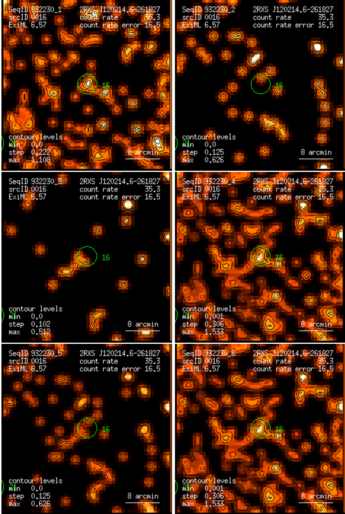
Figure 16: RASS 932230: detection 0016: band rate images, Gaussian filter: (1) PSPC channels 11 – 41, (2) 52 – 90, (3) 91 – 201, (4) 11 – 235, (5) 52 – 201, (6) 11 – 201. Broad band rates in counts/ks. Band rate contour levels in counts/ks/arcmin 2 .
