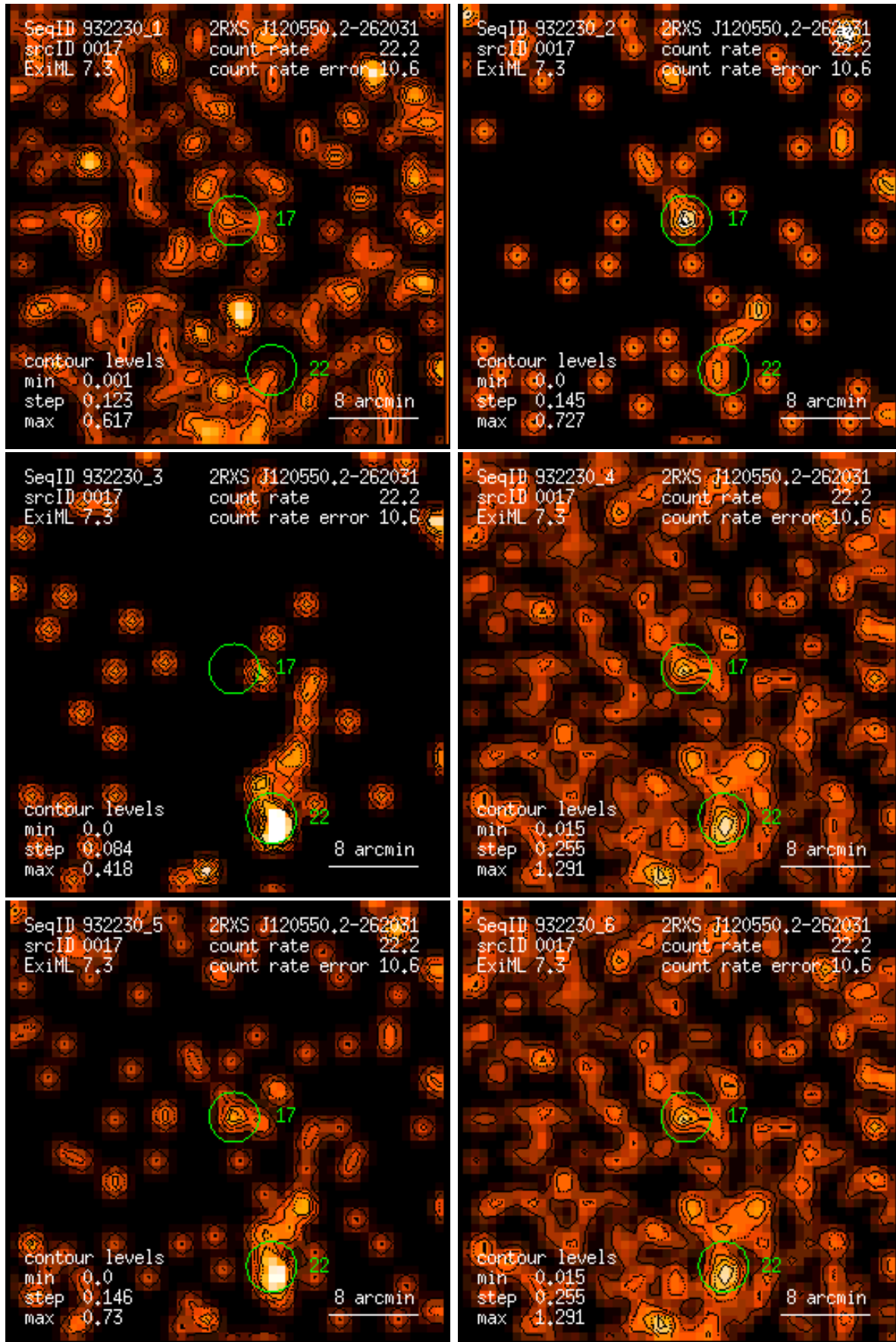
Figure 17: RASS 932230: detection 0017: band rate images, Gaussian filter: (1) PSPC channels 11 – 41, (2) 52 – 90, (3) 91 – 201, (4) 11 – 235, (5) 52 – 201, (6) 11 – 201. Broad band rates in counts/ks. Band rate contour levels in counts/ks/arcmin 2 .
