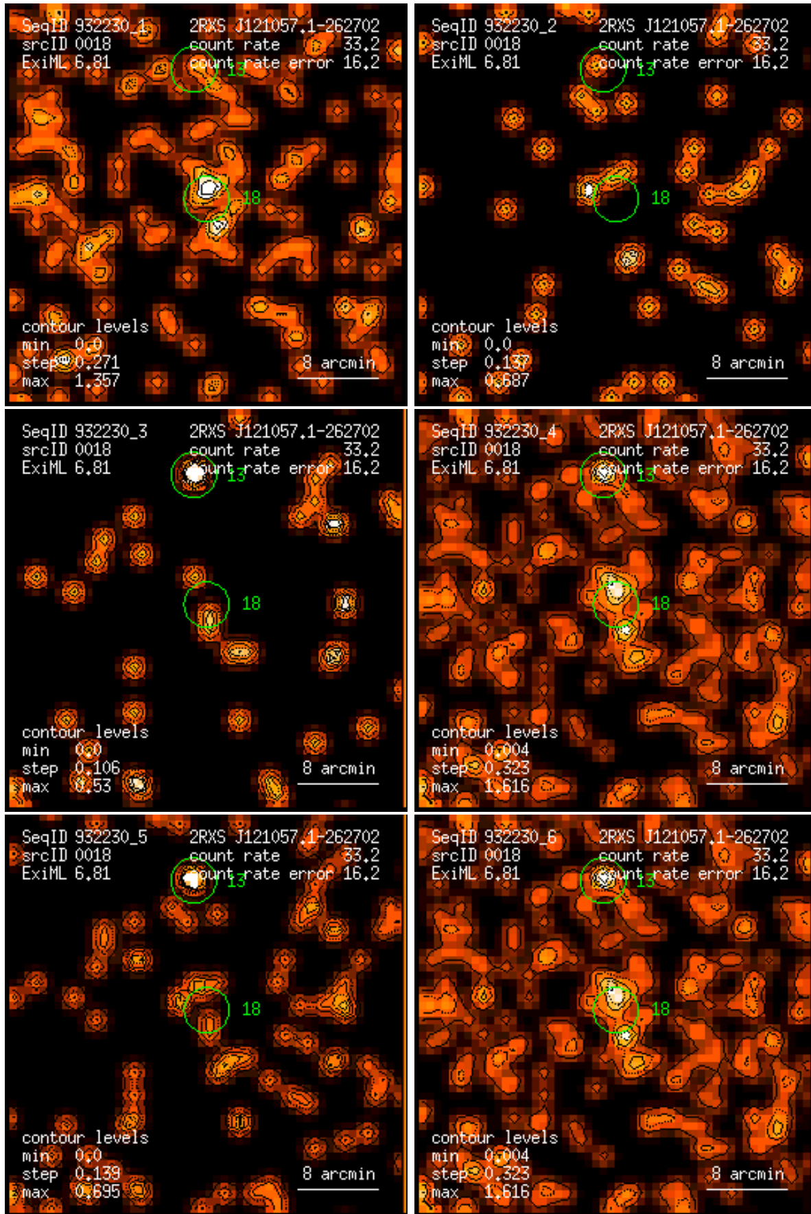
Figure 18: RASS 932230: detection 0018: band rate images, Gaussian filter: (1) PSPC channels 11 – 41, (2) 52 – 90, (3) 91 – 201, (4) 11 – 235, (5) 52 – 201, (6) 11 – 201. Broad band rates in counts/ks. Band rate contour levels in counts/ks/arcmin 2 .
