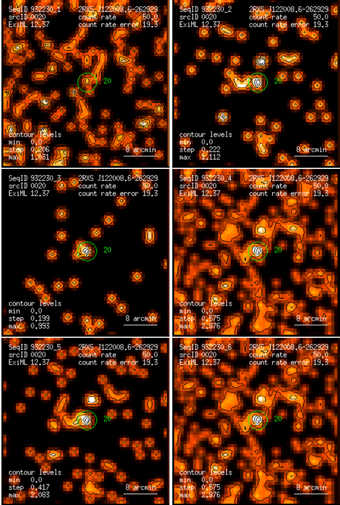
Figure 20: RASS 932230: detection 0020: band rate images, Gaussian filter: (1) PSPC channels 11 – 41, (2) 52 – 90, (3) 91 – 201, (4) 11 – 235, (5) 52 – 201, (6) 11 – 201. Broad band rates in counts/ks. Band rate contour levels in counts/ks/arcmin 2 .
