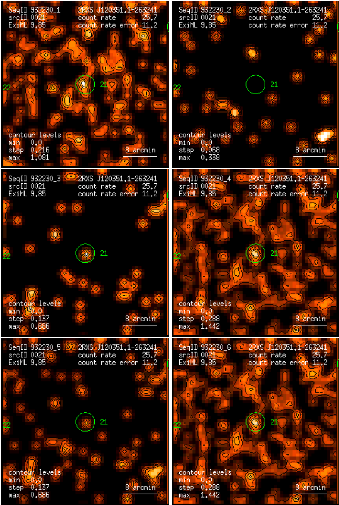
Figure 21: RASS 932230: detection 0021: band rate images, Gaussian filter: (1) PSPC channels 11 – 41, (2) 52 – 90, (3) 91 – 201, (4) 11 – 235, (5) 52 – 201, (6) 11 – 201. Broad band rates in counts/ks. Band rate contour levels in counts/ks/arcmin 2 .
