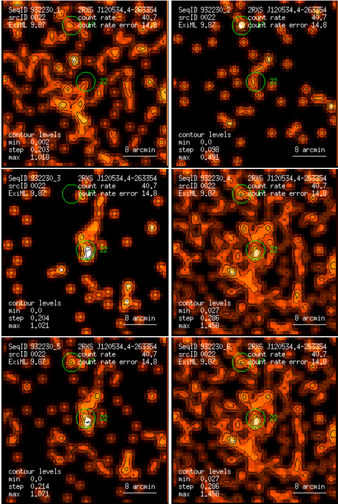
Figure 22: RASS 932230: detection 0022: band rate images, Gaussian filter: (1) PSPC channels 11 – 41, (2) 52 – 90, (3) 91 – 201, (4) 11 – 235, (5) 52 – 201, (6) 11 – 201. Broad band rates in counts/ks. Band rate contour levels in counts/ks/arcmin 2 .
