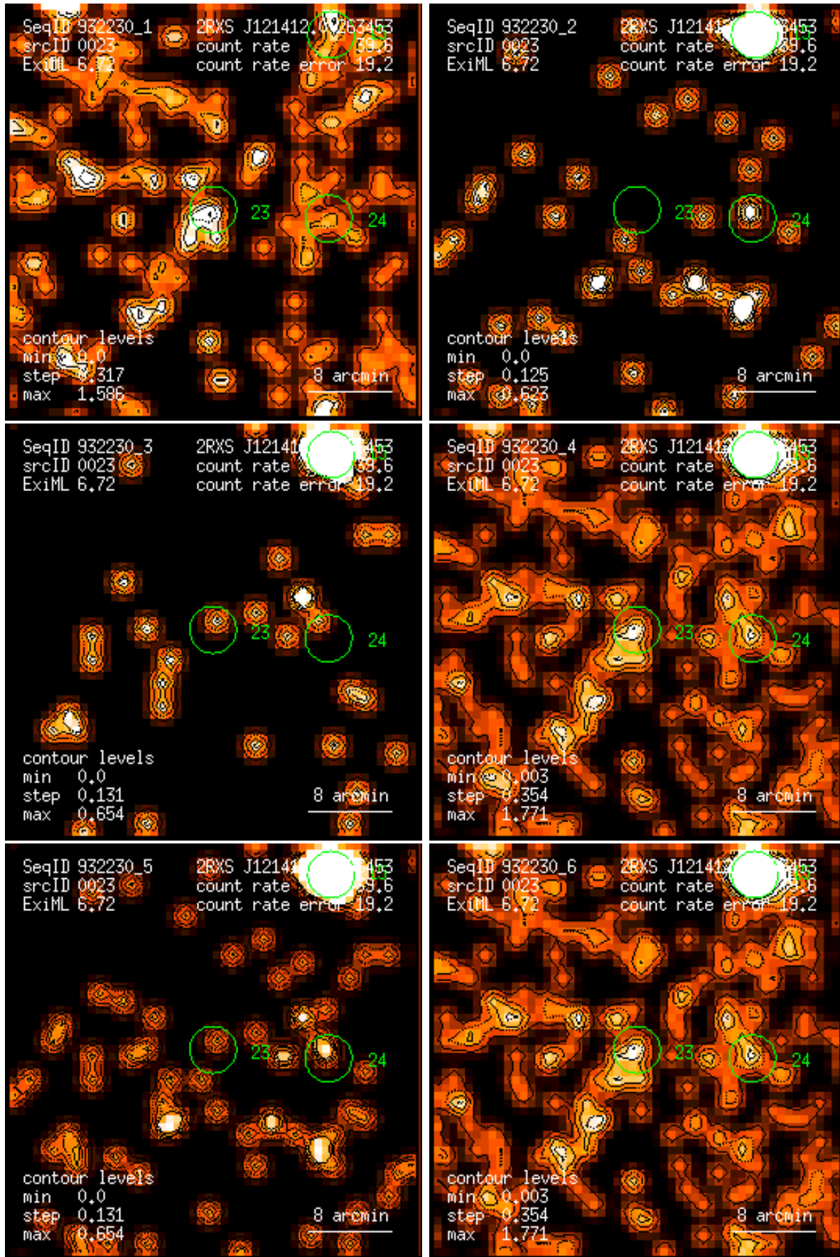
Figure 23: RASS 932230: detection 0023: band rate images, Gaussian filter: (1) PSPC channels 11 – 41, (2) 52 – 90, (3) 91 – 201, (4) 11 – 235, (5) 52 – 201, (6) 11 – 201. Broad band rates in counts/ks. Band rate contour levels in counts/ks/arcmin 2 .
