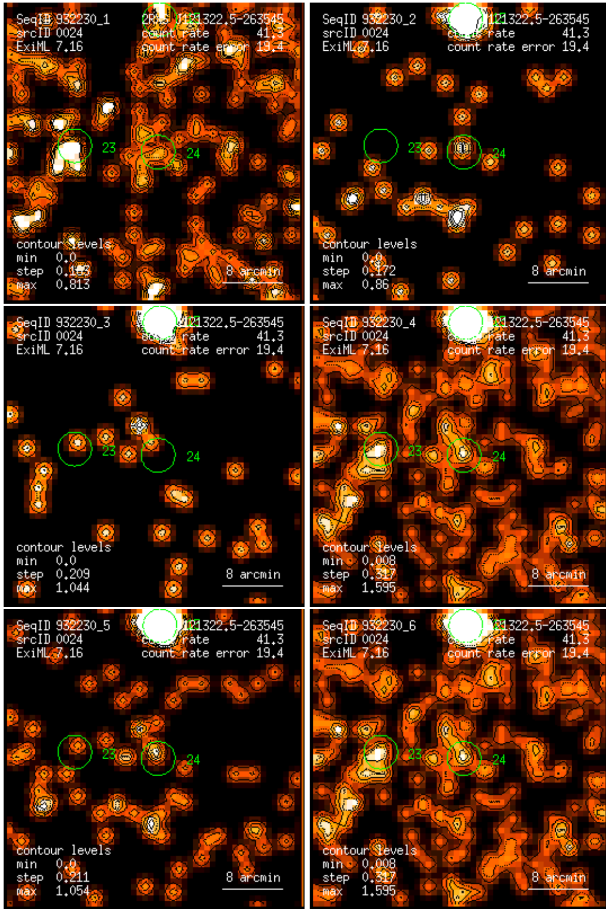
Figure 24: RASS 932230: detection 0024: band rate images, Gaussian filter: (1) PSPC channels 11 – 41, (2) 52 – 90, (3) 91 – 201, (4) 11 – 235, (5) 52 – 201, (6) 11 – 201. Broad band rates in counts/ks. Band rate contour levels in counts/ks/arcmin 2 .
