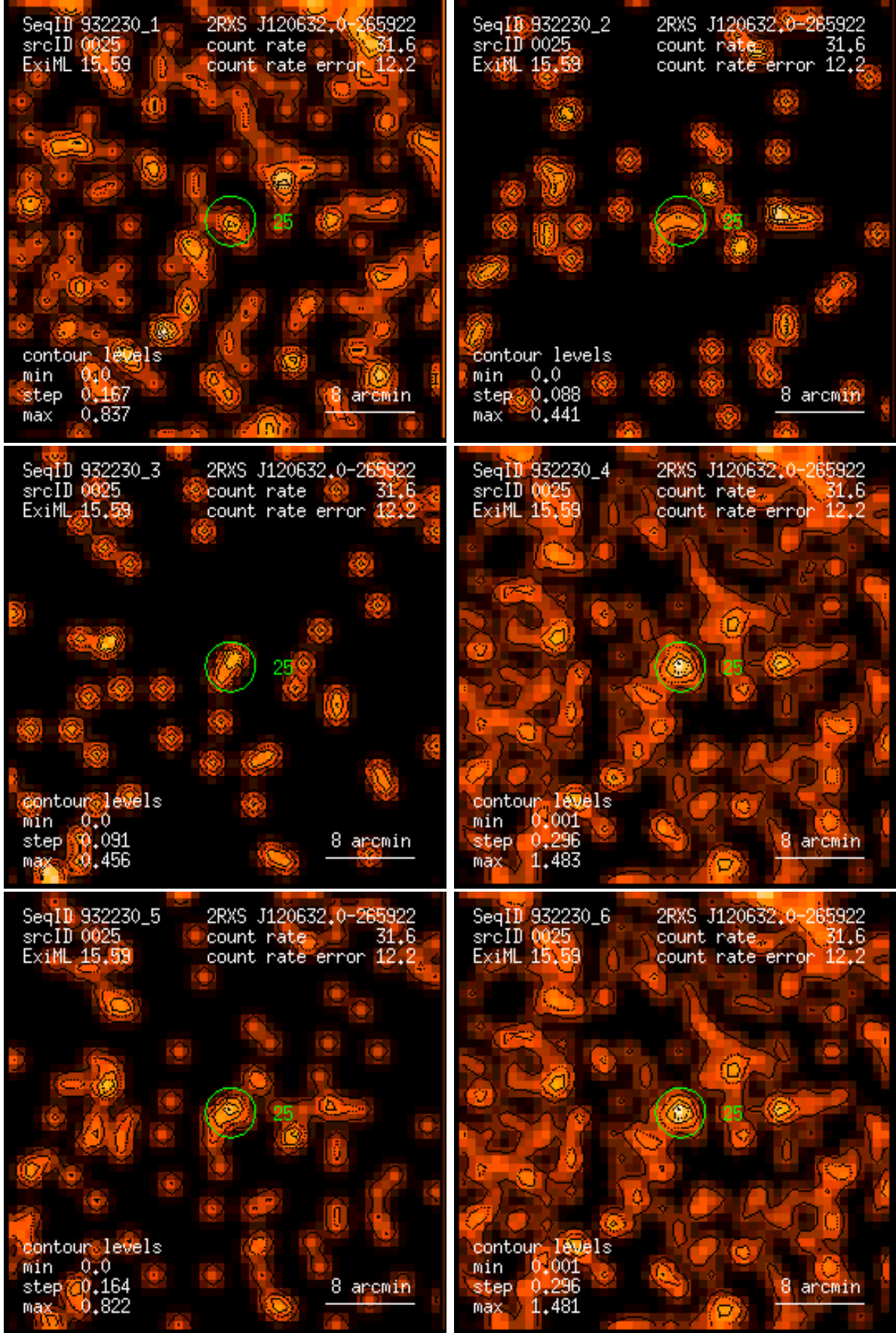
Figure 25: RASS 932230: detection 0025: band rate images, Gaussian filter: (1) PSPC channels 11 – 41, (2) 52 – 90, (3) 91 – 201, (4) 11 – 235, (5) 52 – 201, (6) 11 – 201. Broad band rates in counts/ks. Band rate contour levels in counts/ks/arcmin 2 .
