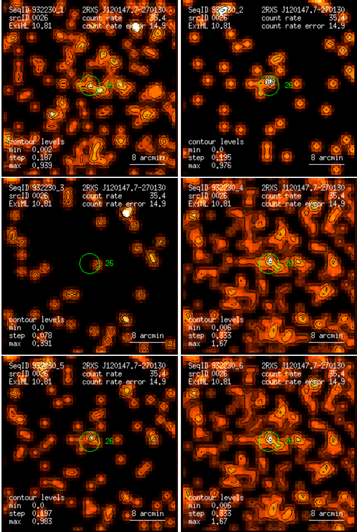
Figure 26: RASS 932230: detection 0026: band rate images, Gaussian filter: (1) PSPC channels 11 – 41, (2) 52 – 90, (3) 91 – 201, (4) 11 – 235, (5) 52 – 201, (6) 11 – 201. Broad band rates in counts/ks. Band rate contour levels in counts/ks/arcmin 2 .
